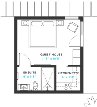
GUEST HOUSE / FOURTH BEDROOM OPTION
