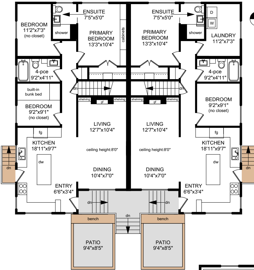
MAIN FLOOR (# 1756) 1056 SQ.FT
