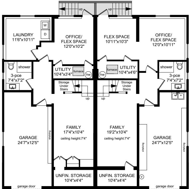
LOWER FLOOR (# 1764) 803 SQ.FT
