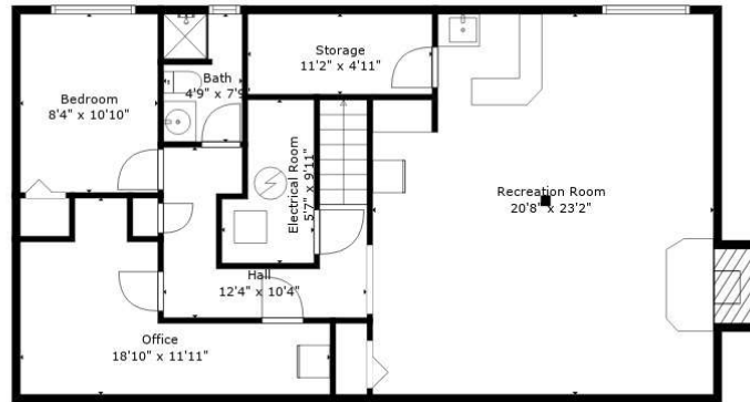
Floor 1
