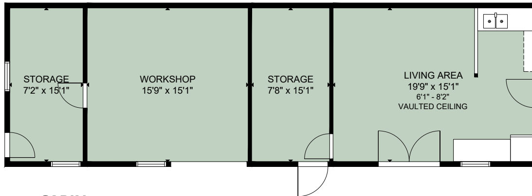
CABIN 765 SQ. FT.
