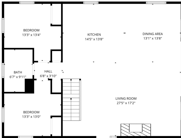
Main Level
