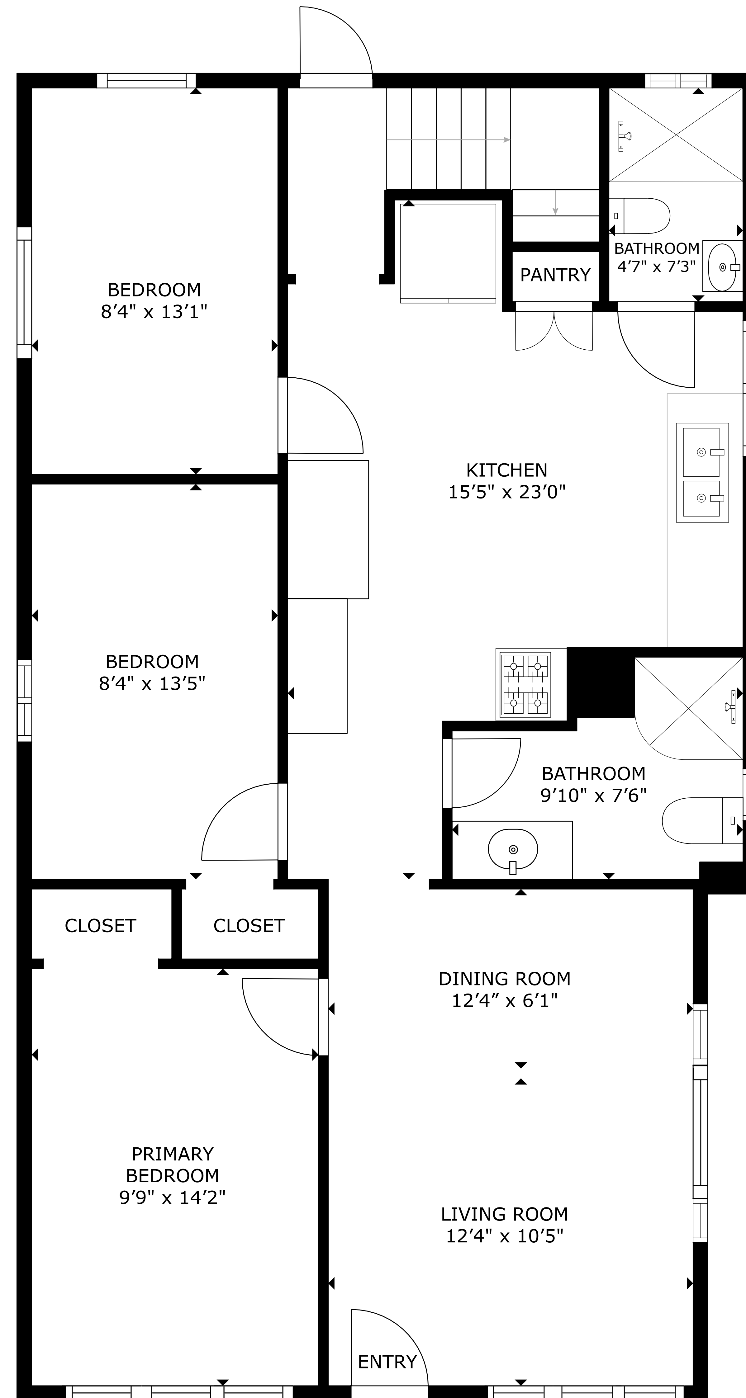
FLOOR 2
