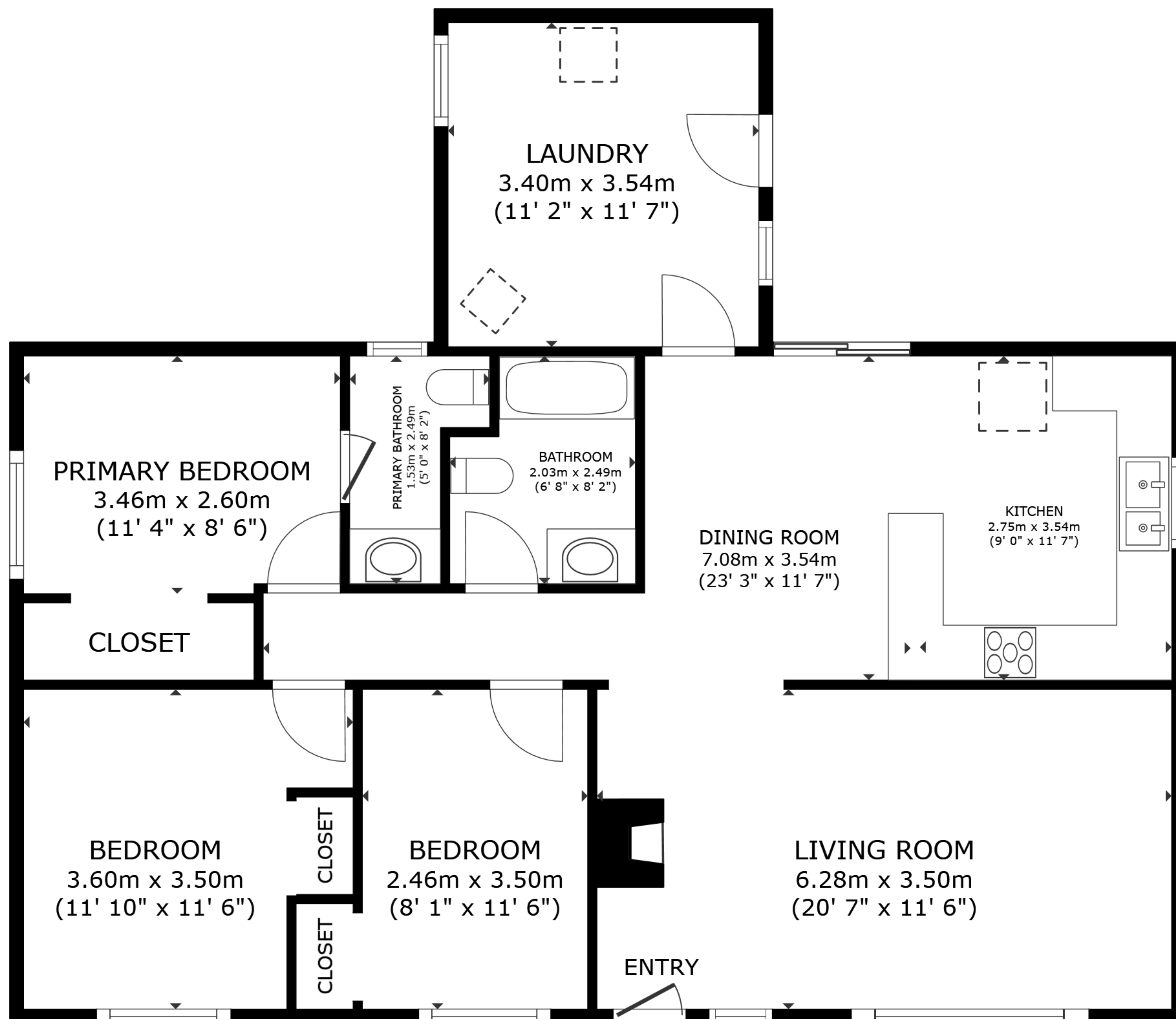
FLOOR PLAN
