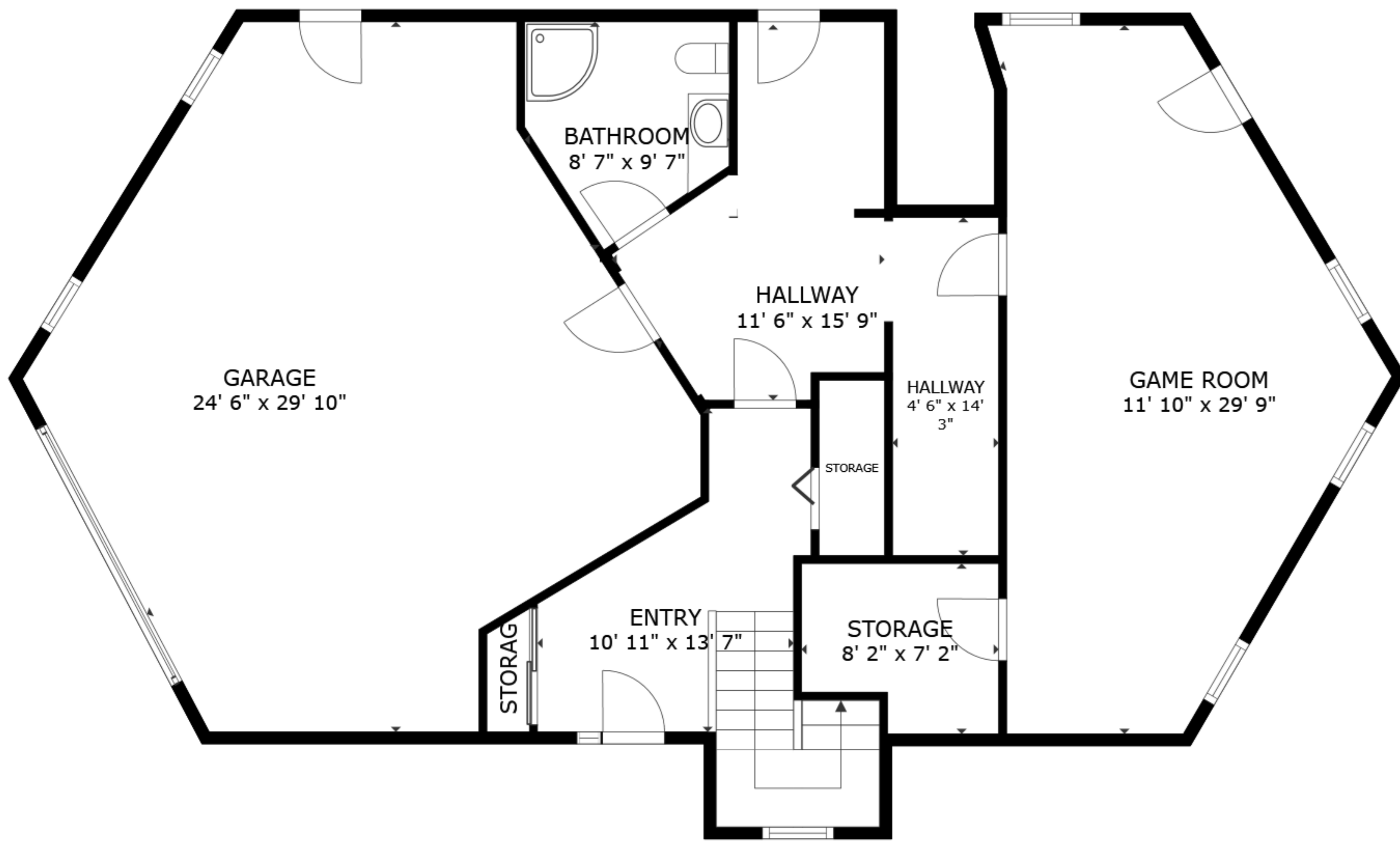
FLOOR 1
