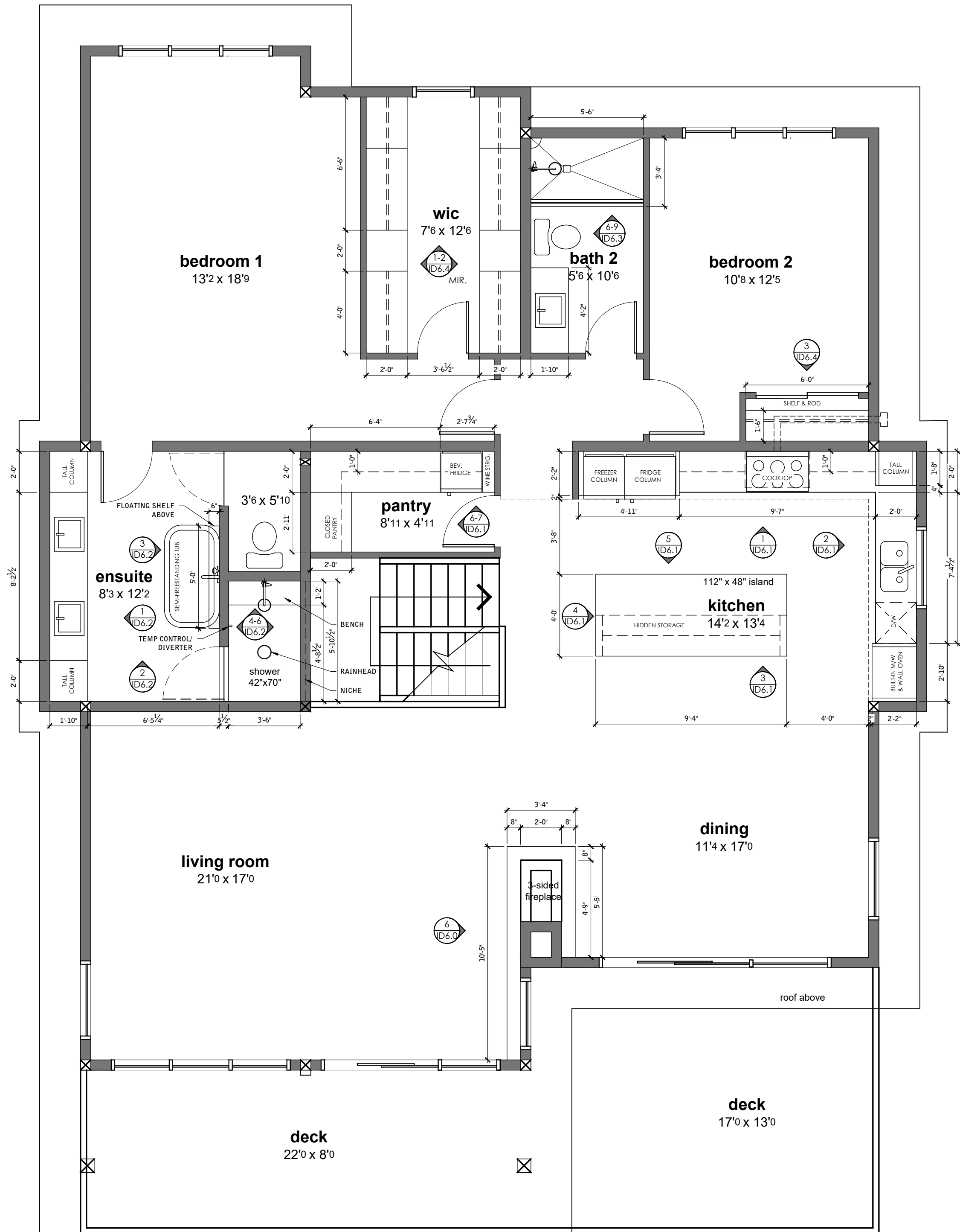
1 MAIN FLOOR - MILLWORK PLAN ID2.1 SCALE: 1/4" = 1'-0"
