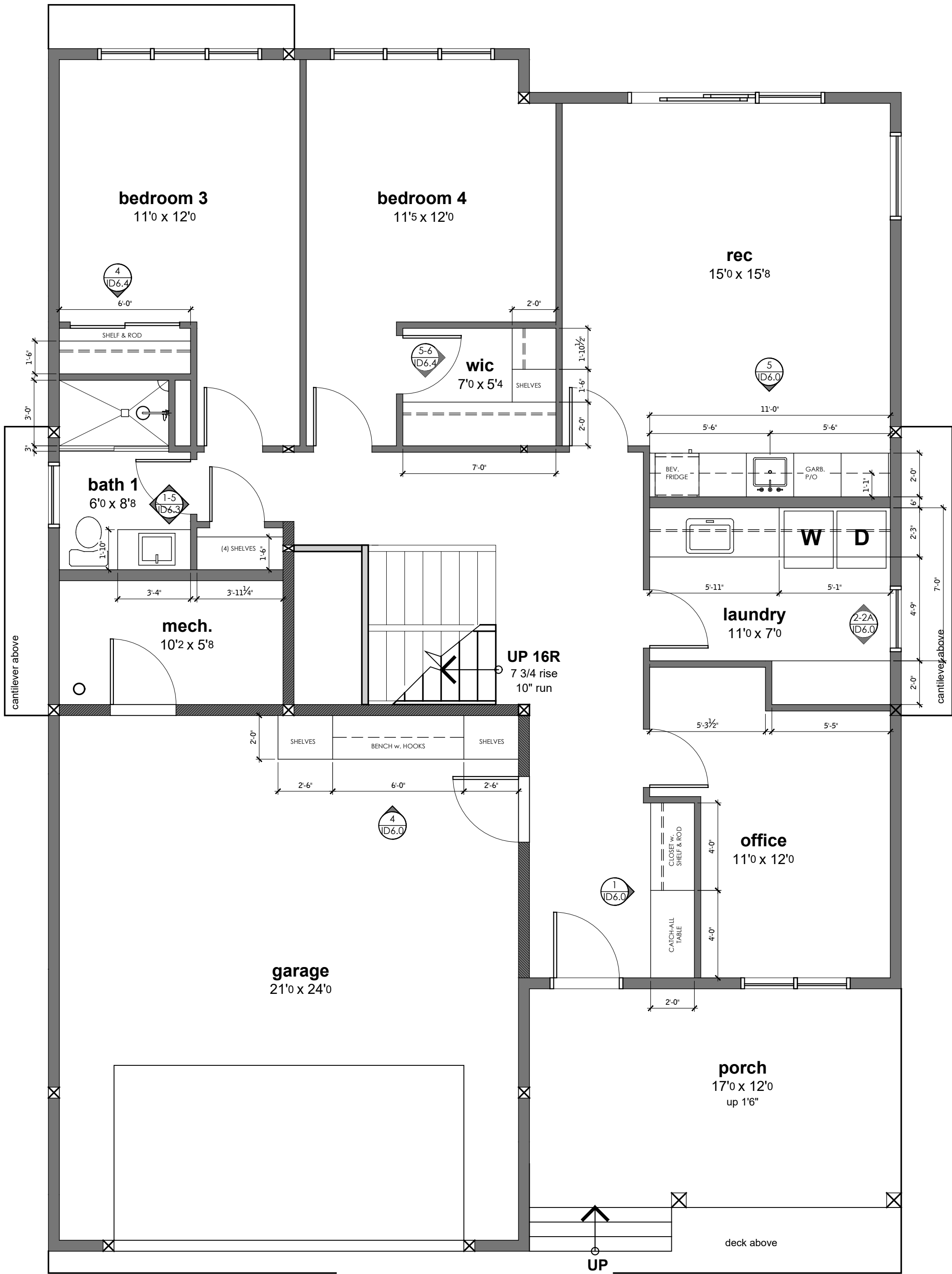
1 LOWER FLOOR - MILLWORK PLAN ID2.0 SCALE: 1/4" = 1'-0"
