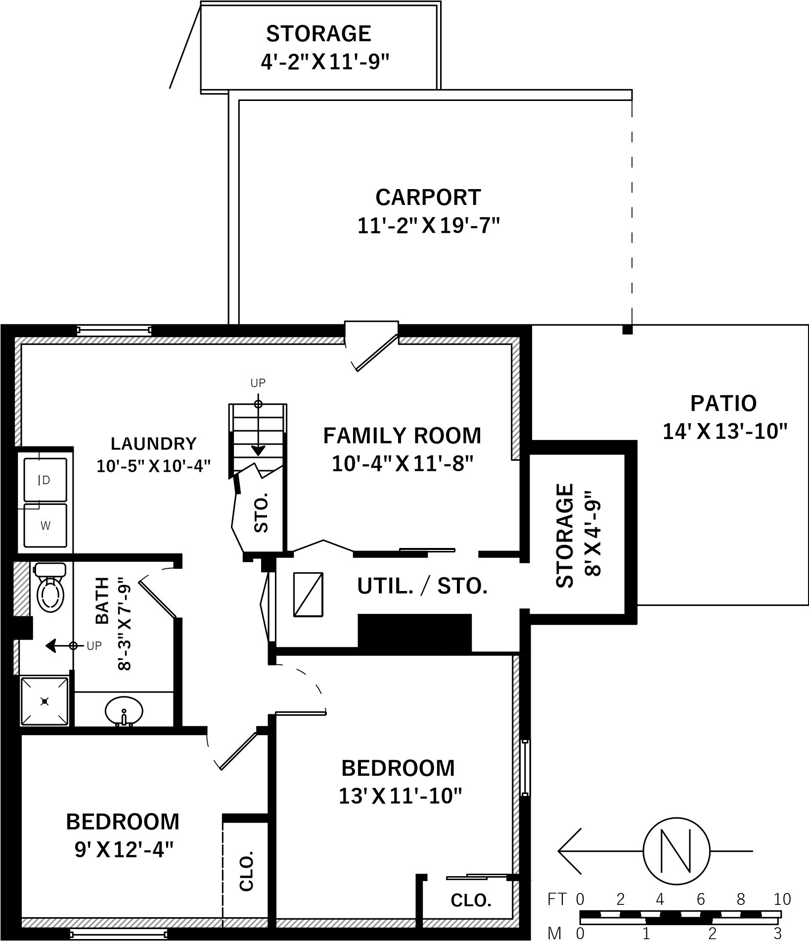
Lower Floor: 853 Sq.Ft. Ceiling Height: 6'-5"
