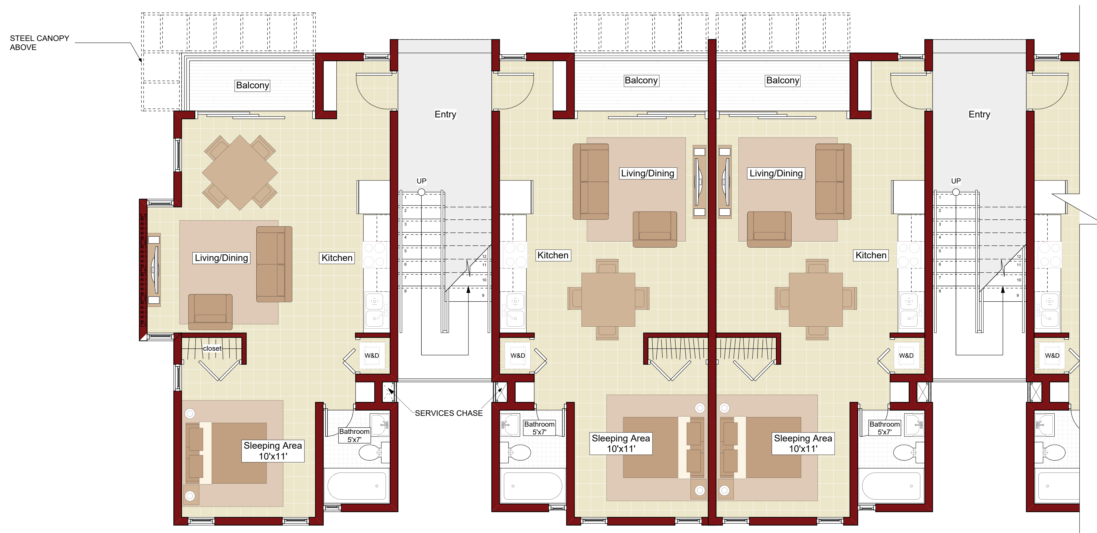
TYPICAL PLAN OF BLOCK "B"
