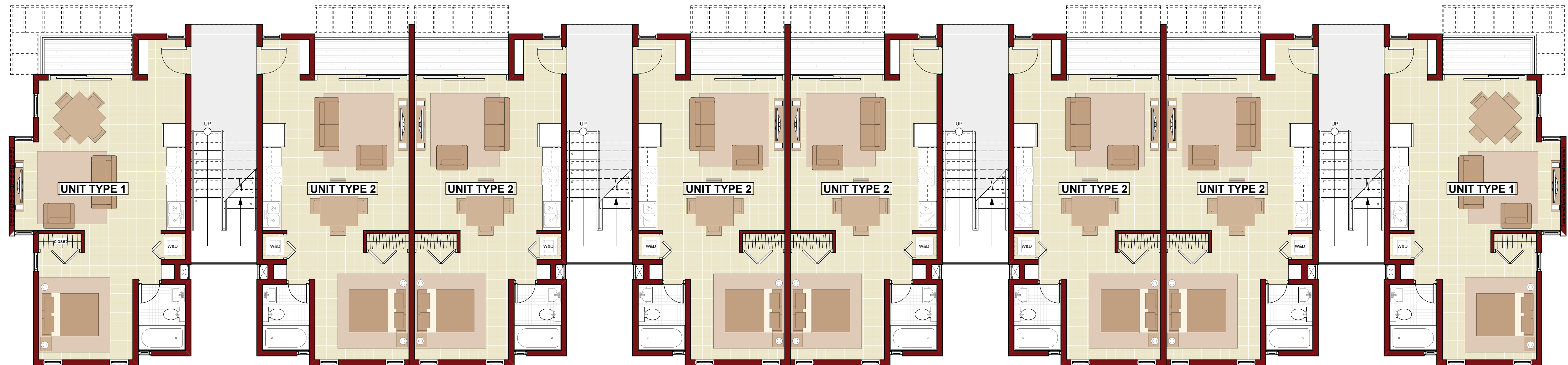
TYPICAL PLAN OF BLOCK "B"
