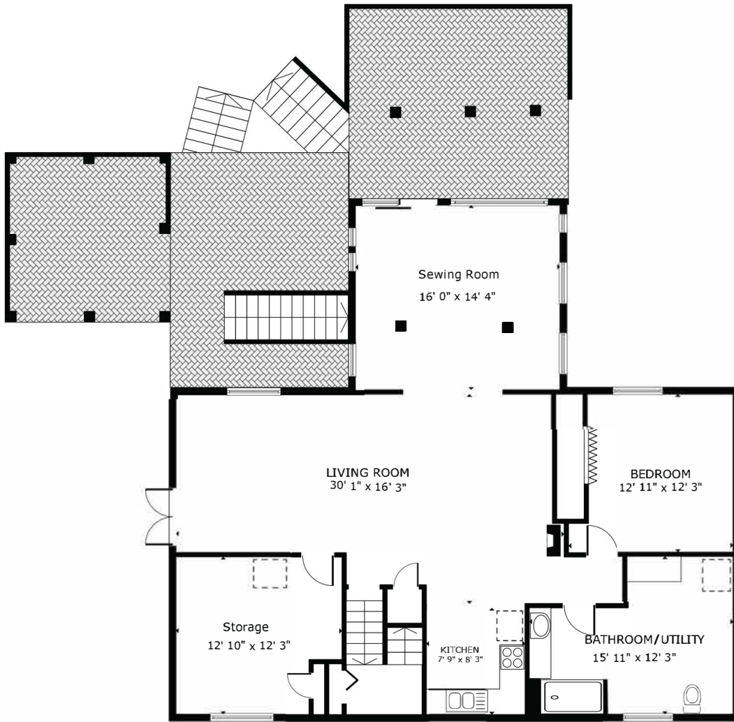
FLOOR 1
