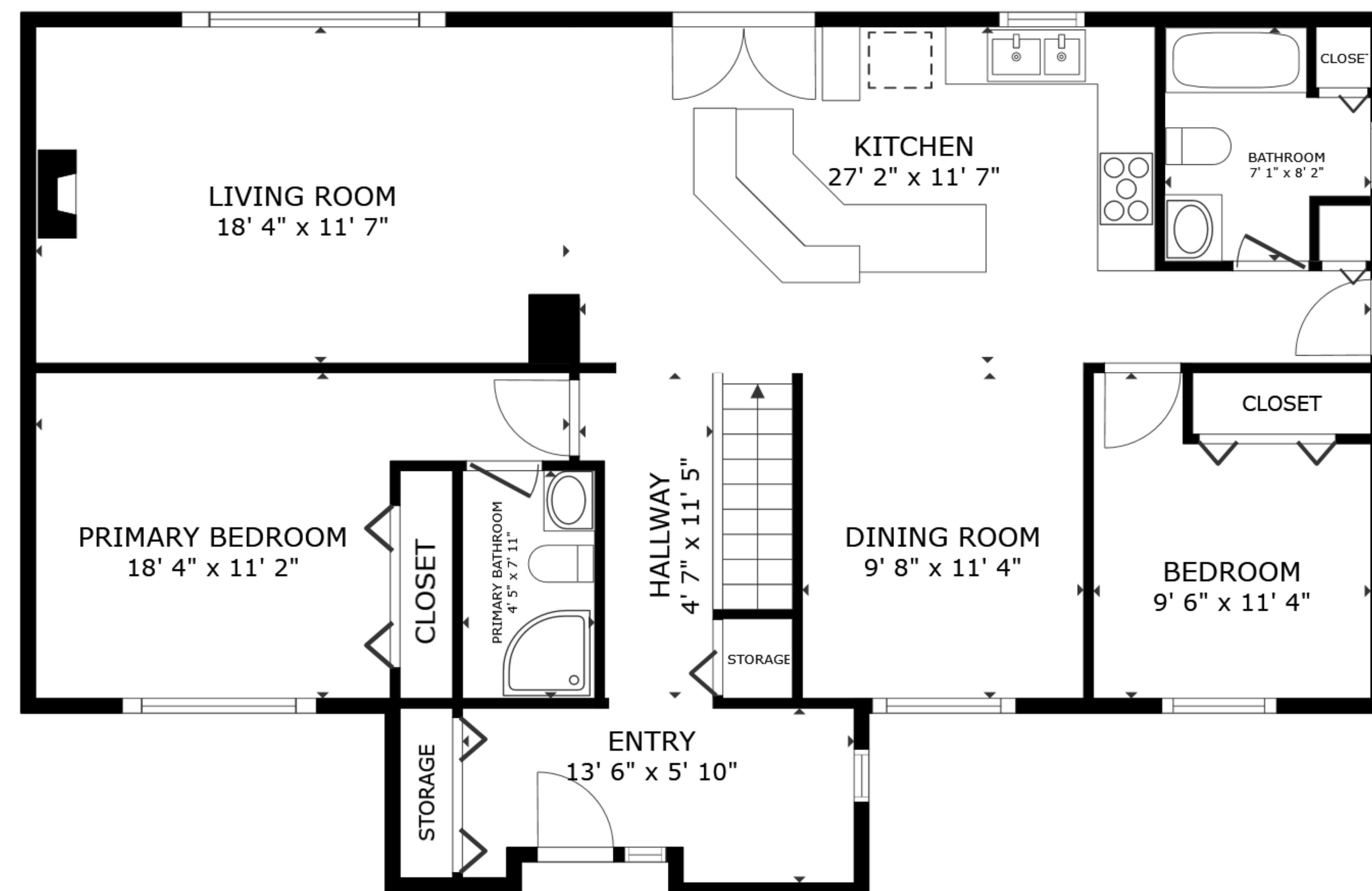
FLOOR 2
