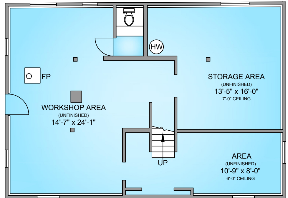
LOWER FLOOR 923 SQ. FT. (UNFINISHED) 6'-0" - 7'-0" CEILING HEIGHT
