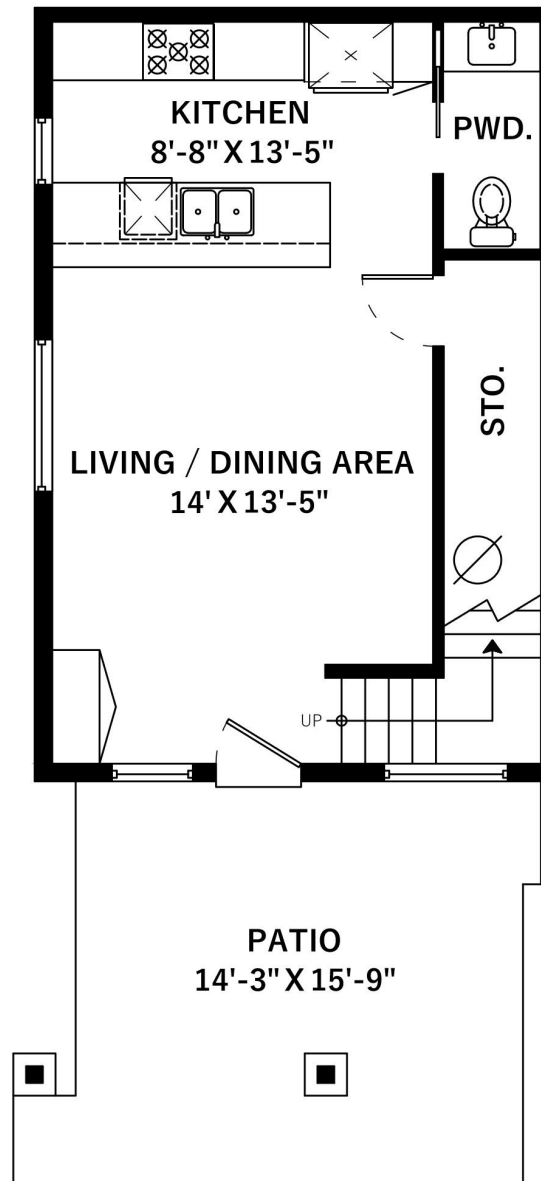
Main Floor: 501 Sq.Ft. Ceiling Height: 9'
