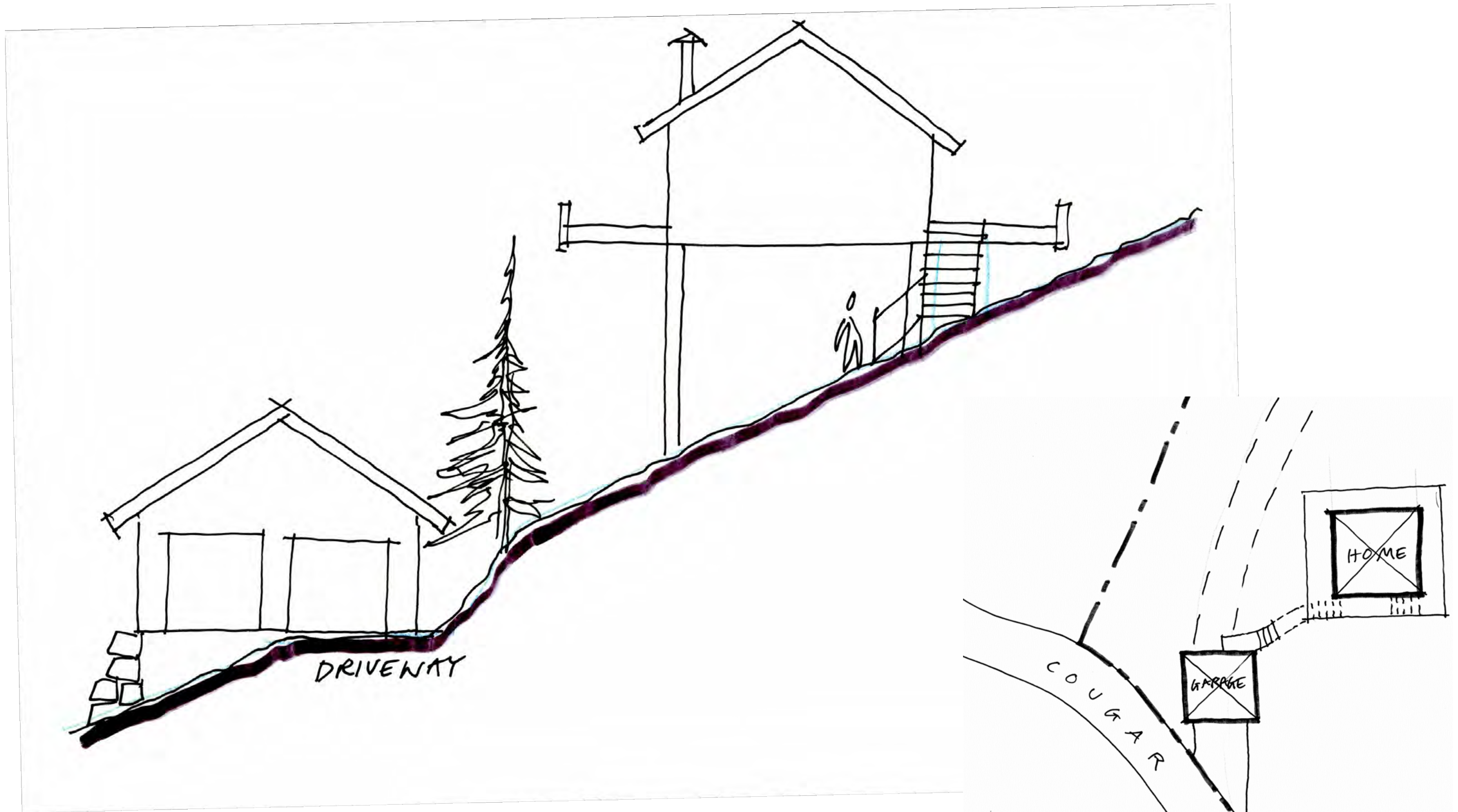
option A - site section & plan
