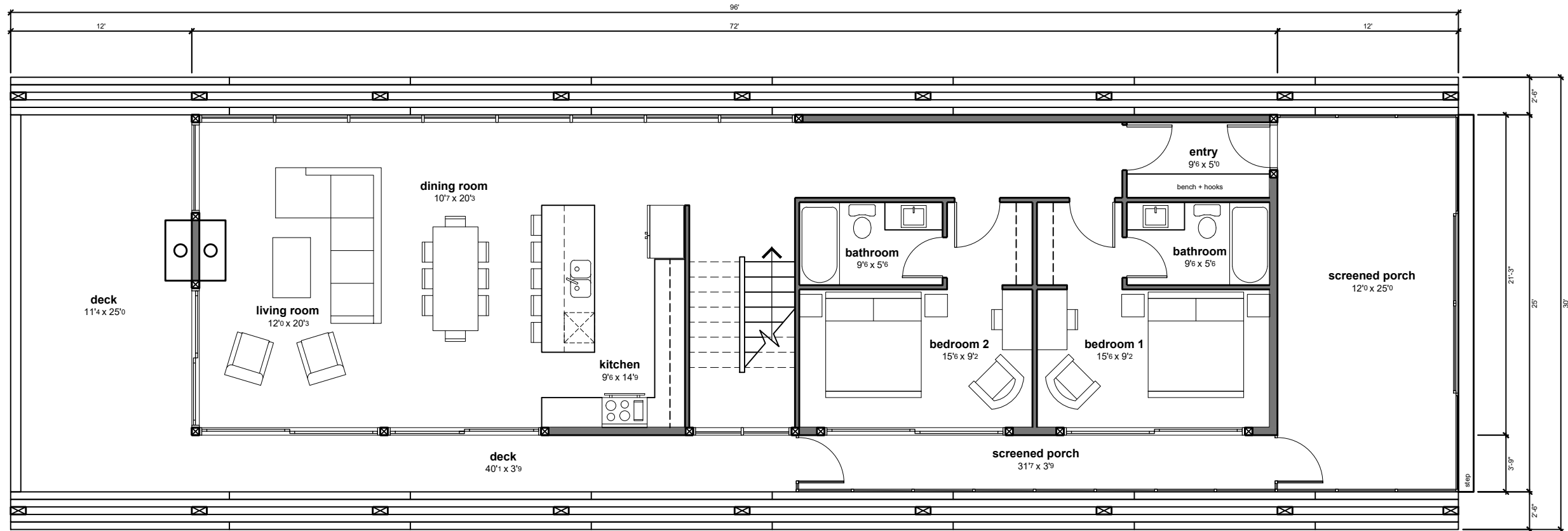
option B - upper floor plan 1438 ft 2
