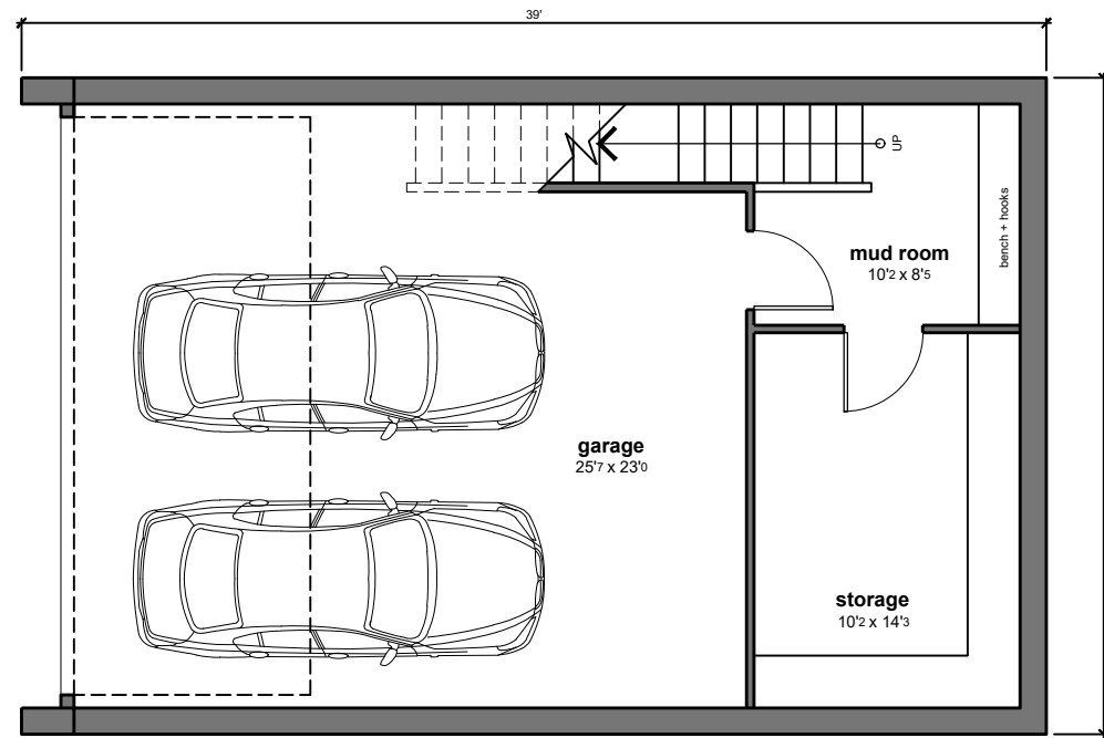
lower floor plan 124 ft 2
