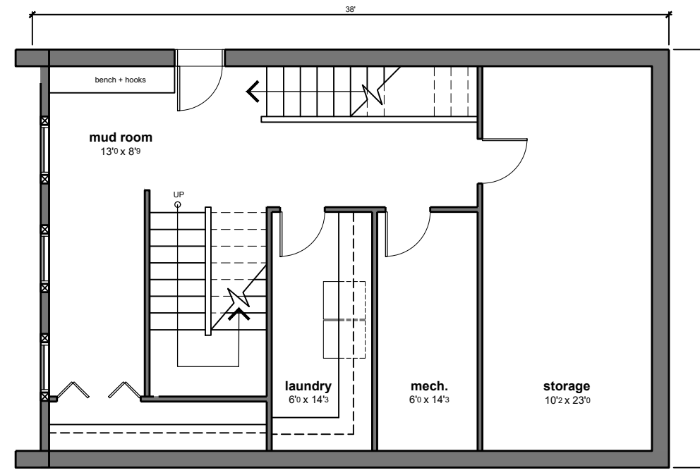
middle floor plan 790 ft 2
