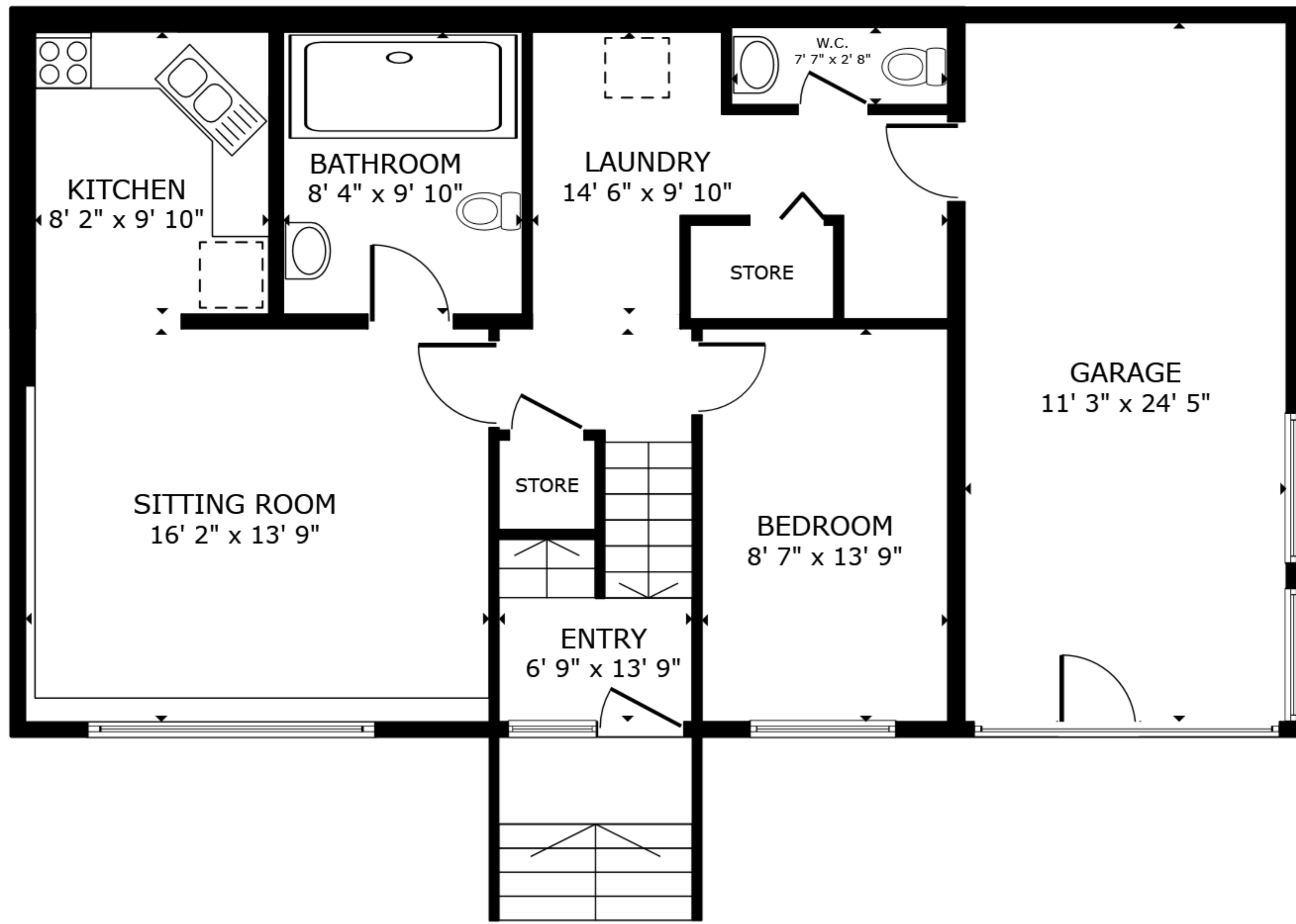
FLOOR 1
