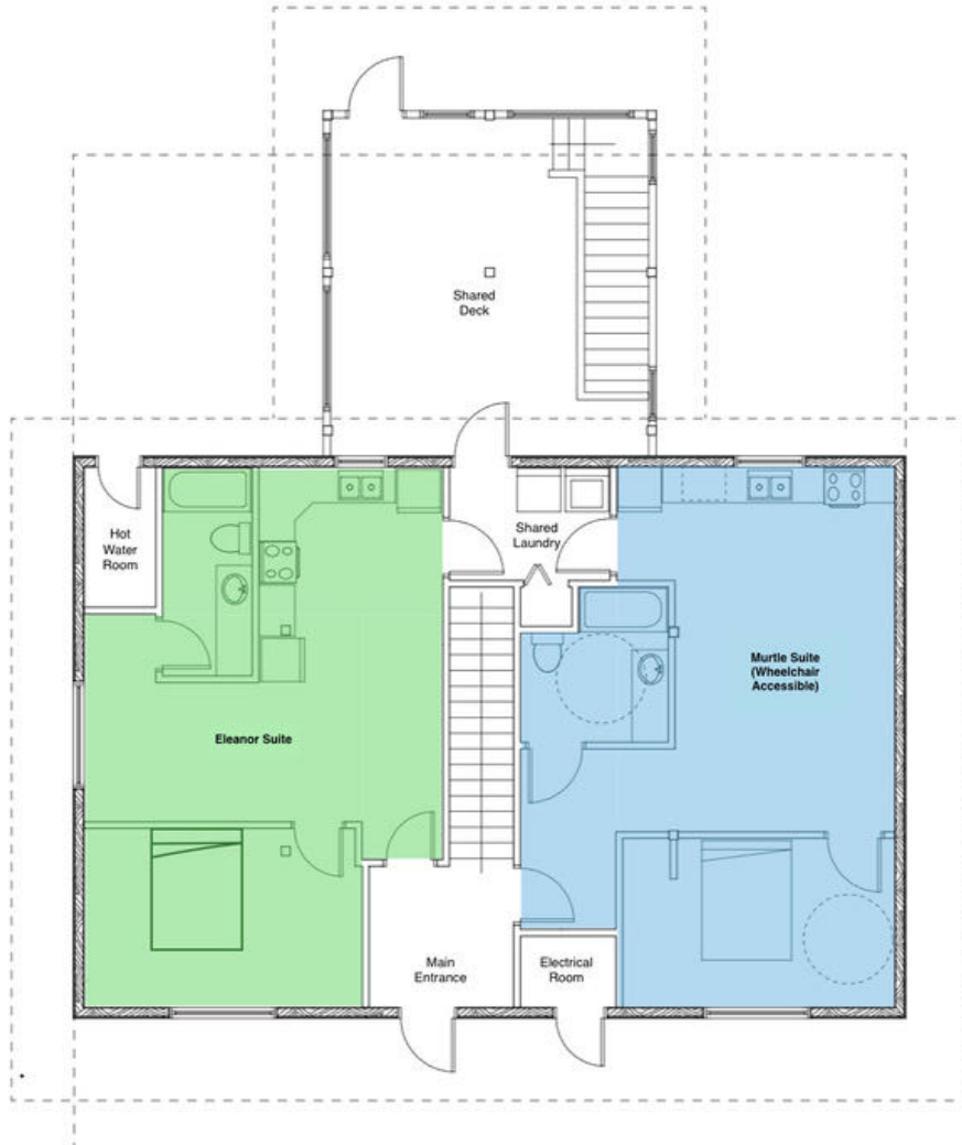
MAIN FLOOR PLAN SCALE: 1/8" = 1'-0"
