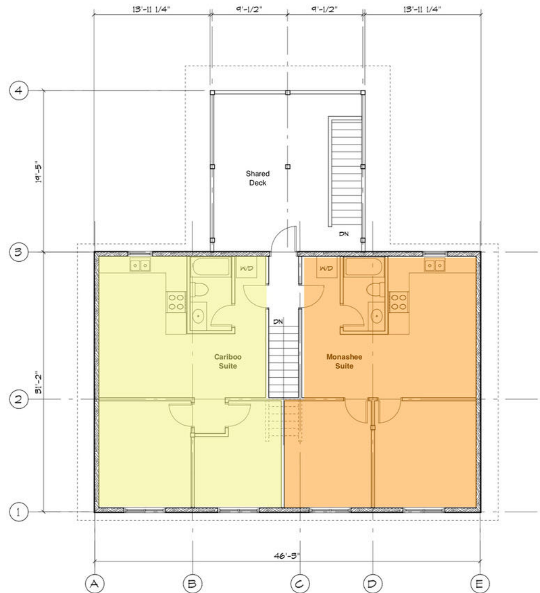
UPPER FLOOR PLAN SCALE: 1/8" = 1'-0"
