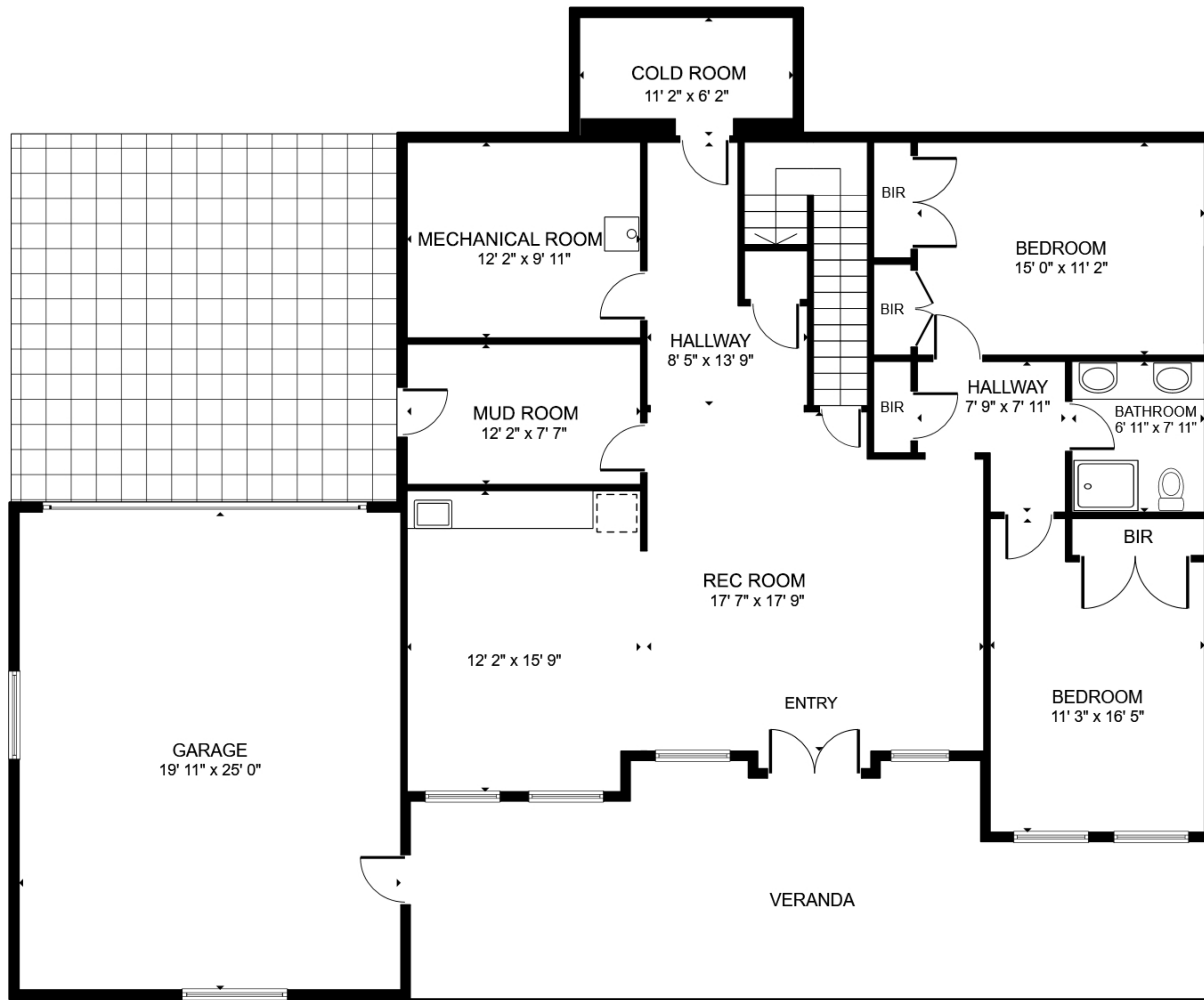
FLOOR 1
