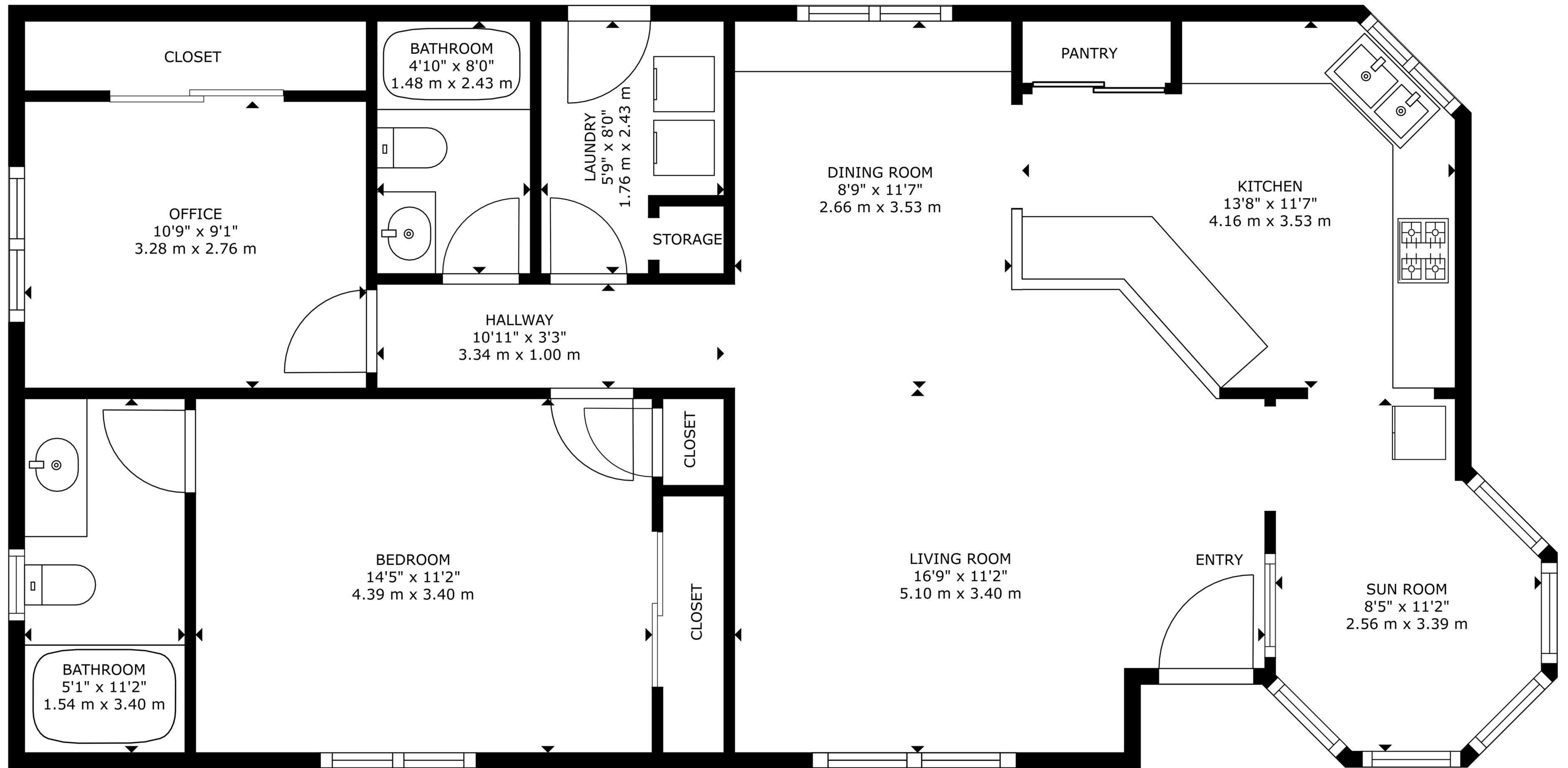
FLOOR PLAN
