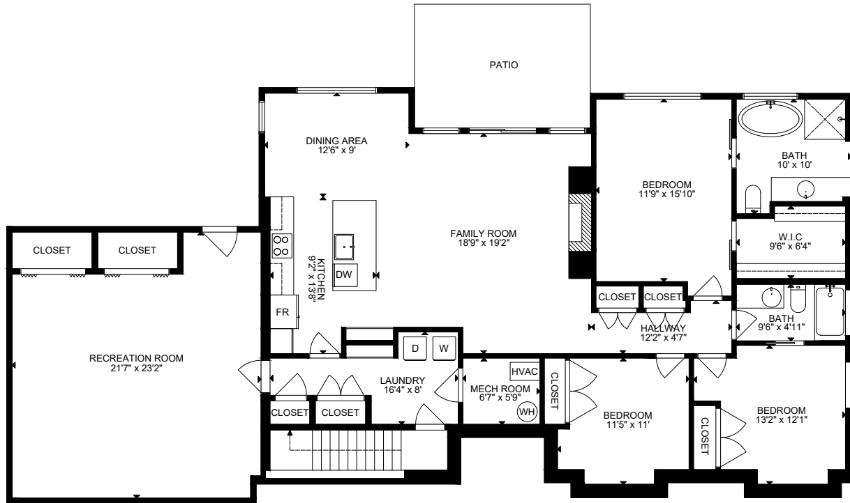
FLOOR 1
