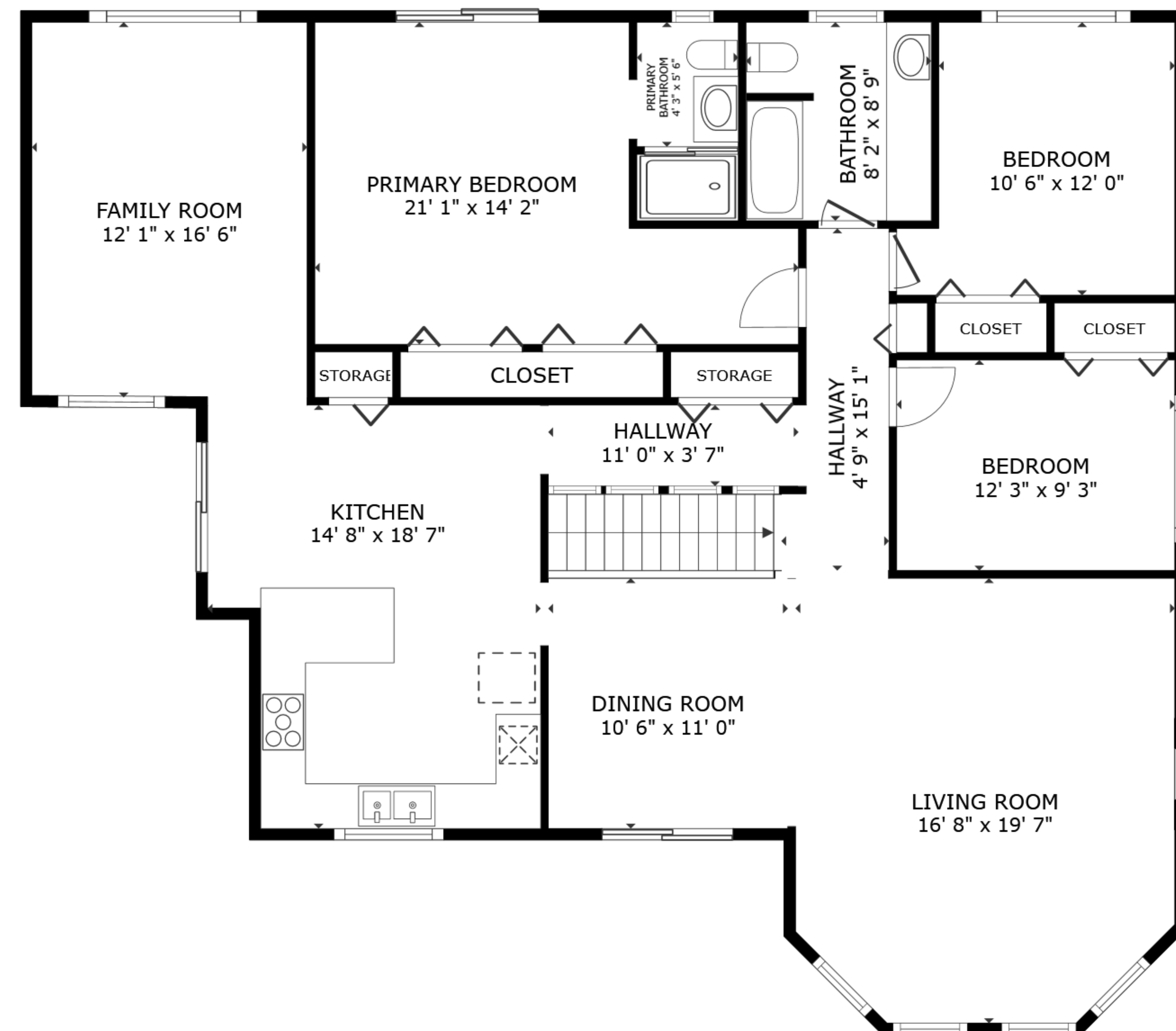
FLOOR 2
