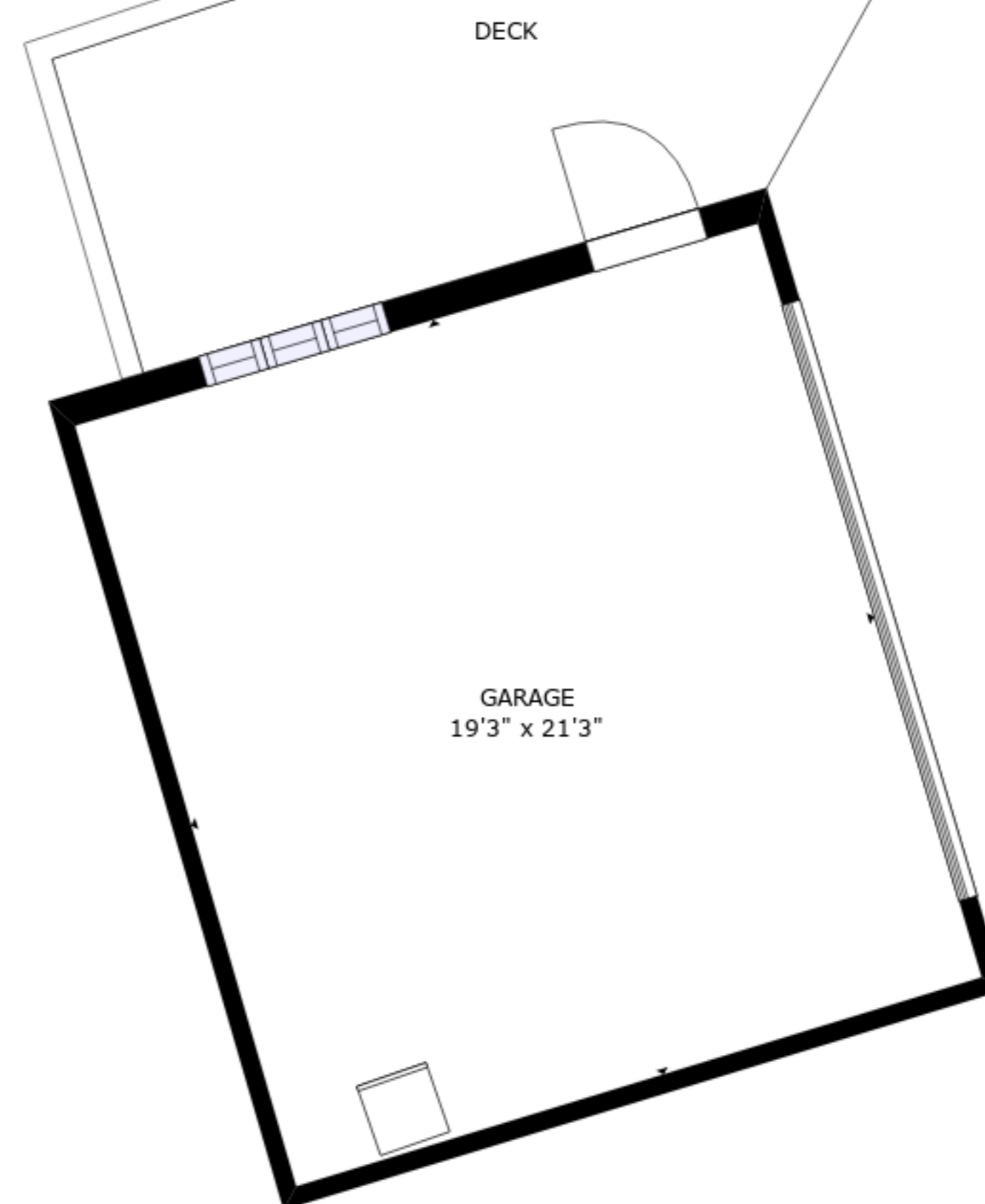
FLOOR 2
