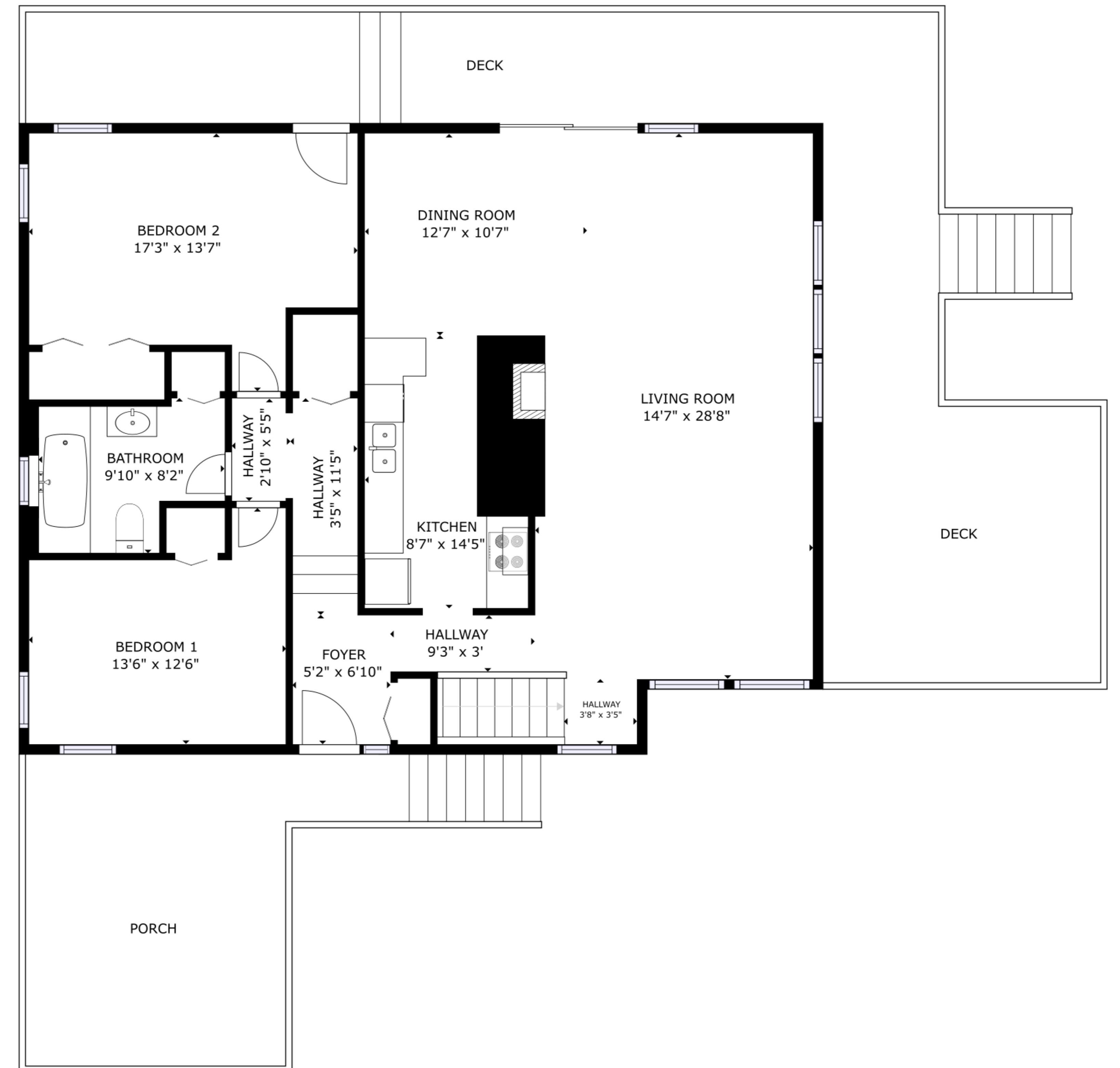
FLOOR 2
