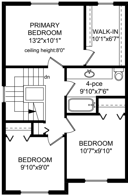
UPPER FLOOR 633 SQ.FT.
