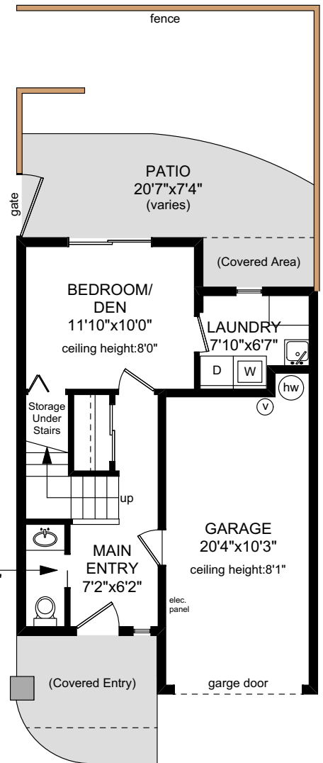
LOWER FLOOR 352 SQ.FT. (Ground Level)
