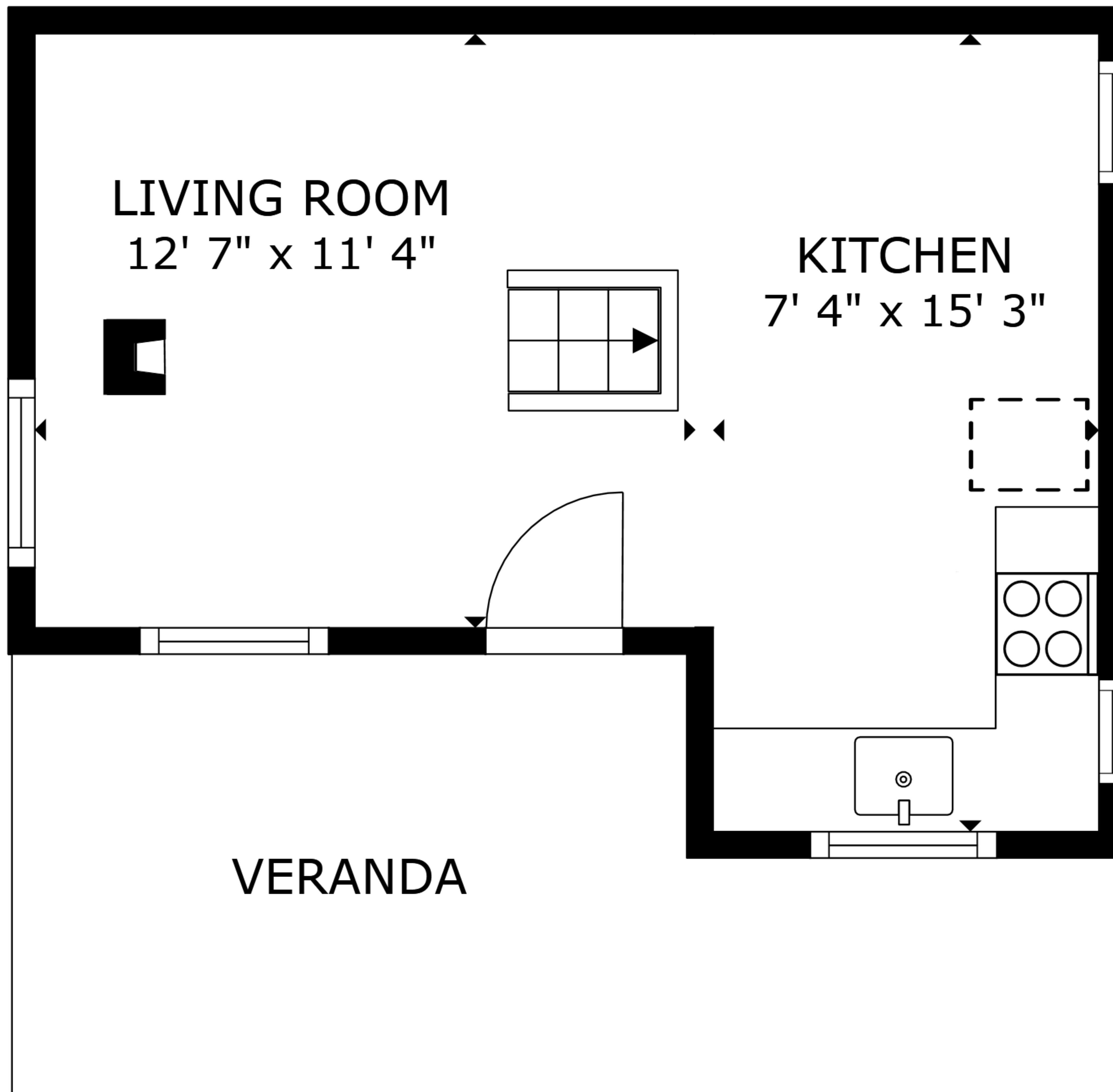
FLOOR 1
