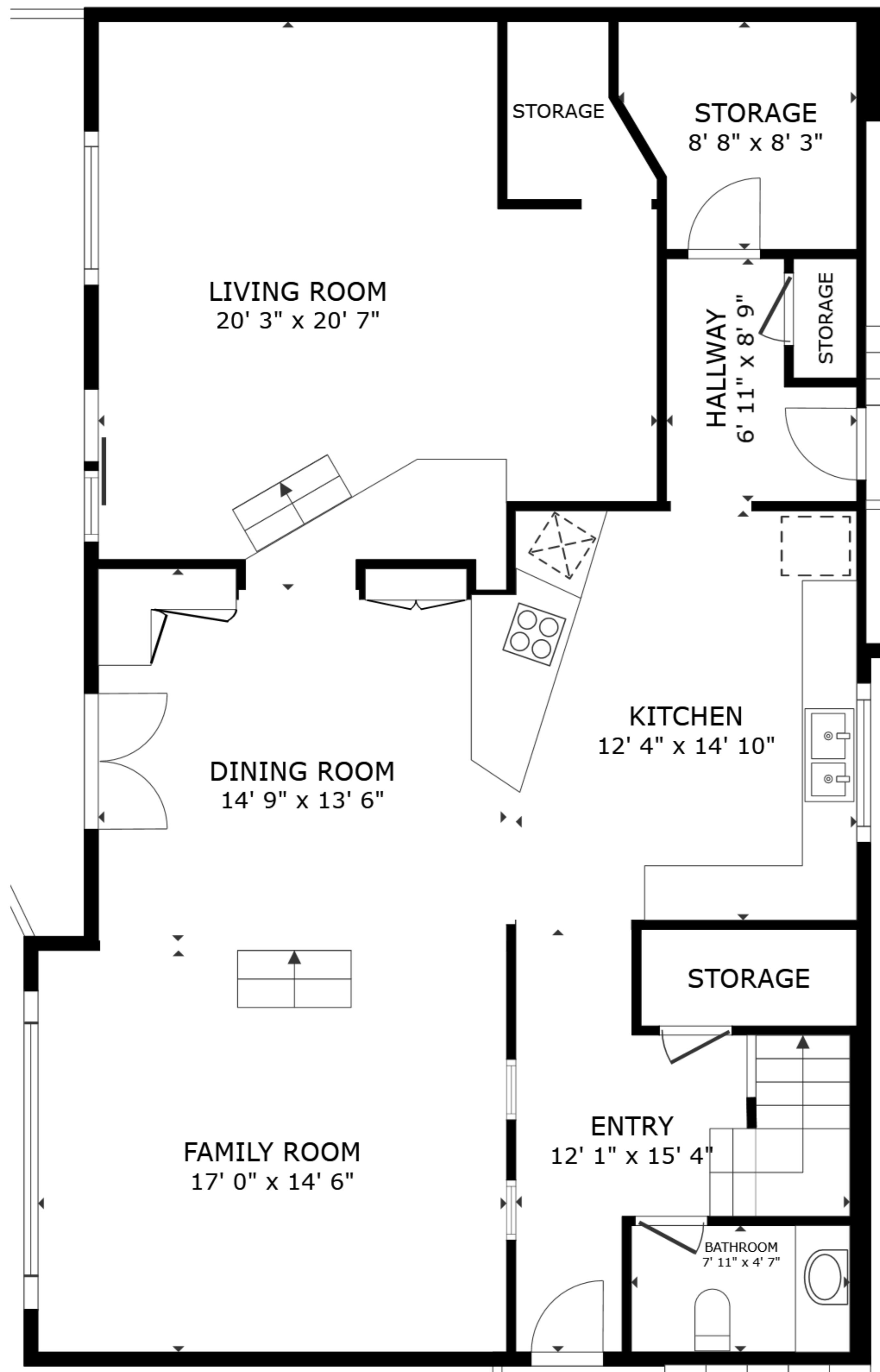
FLOOR 1
