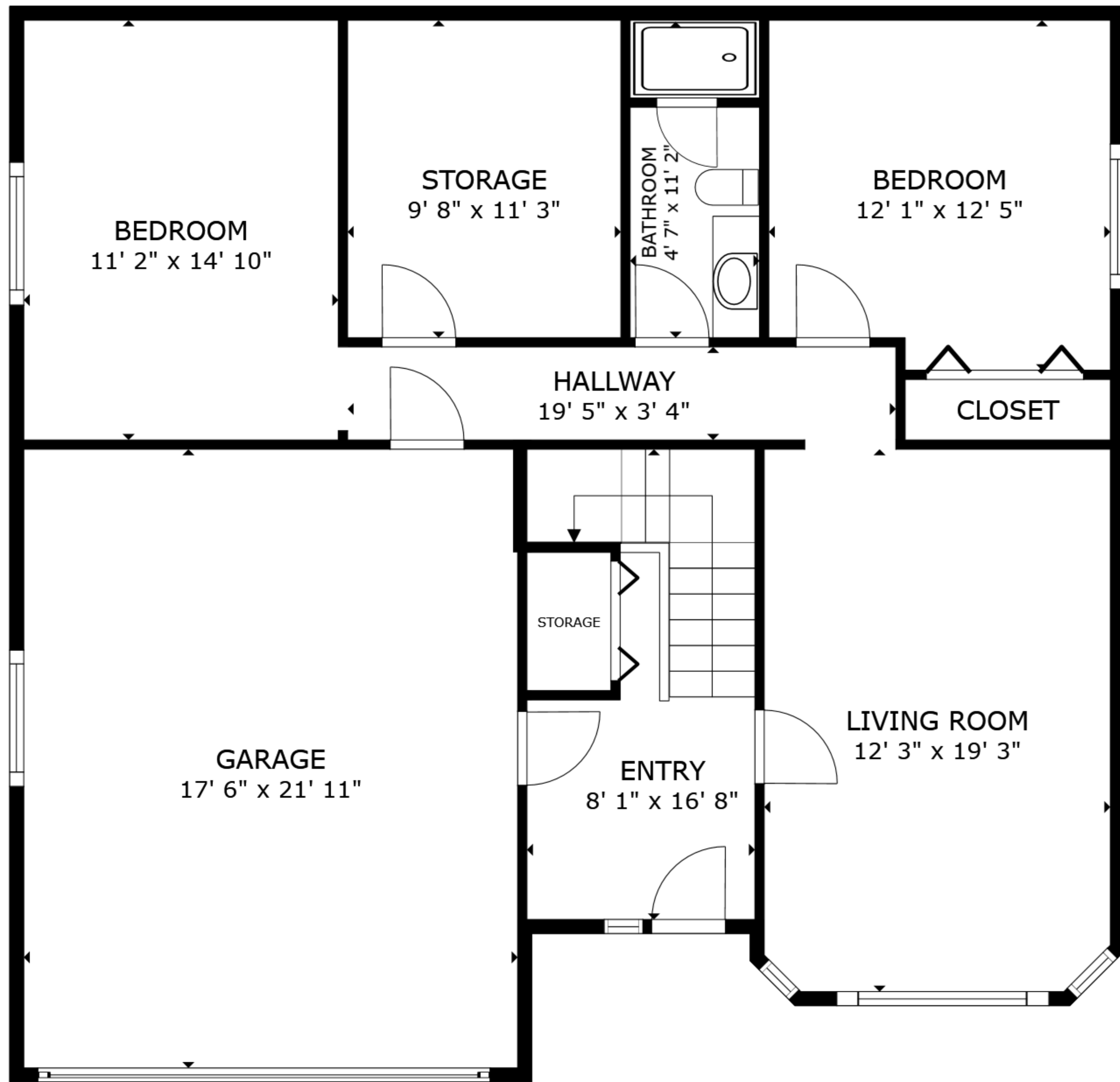
FLOOR 1
