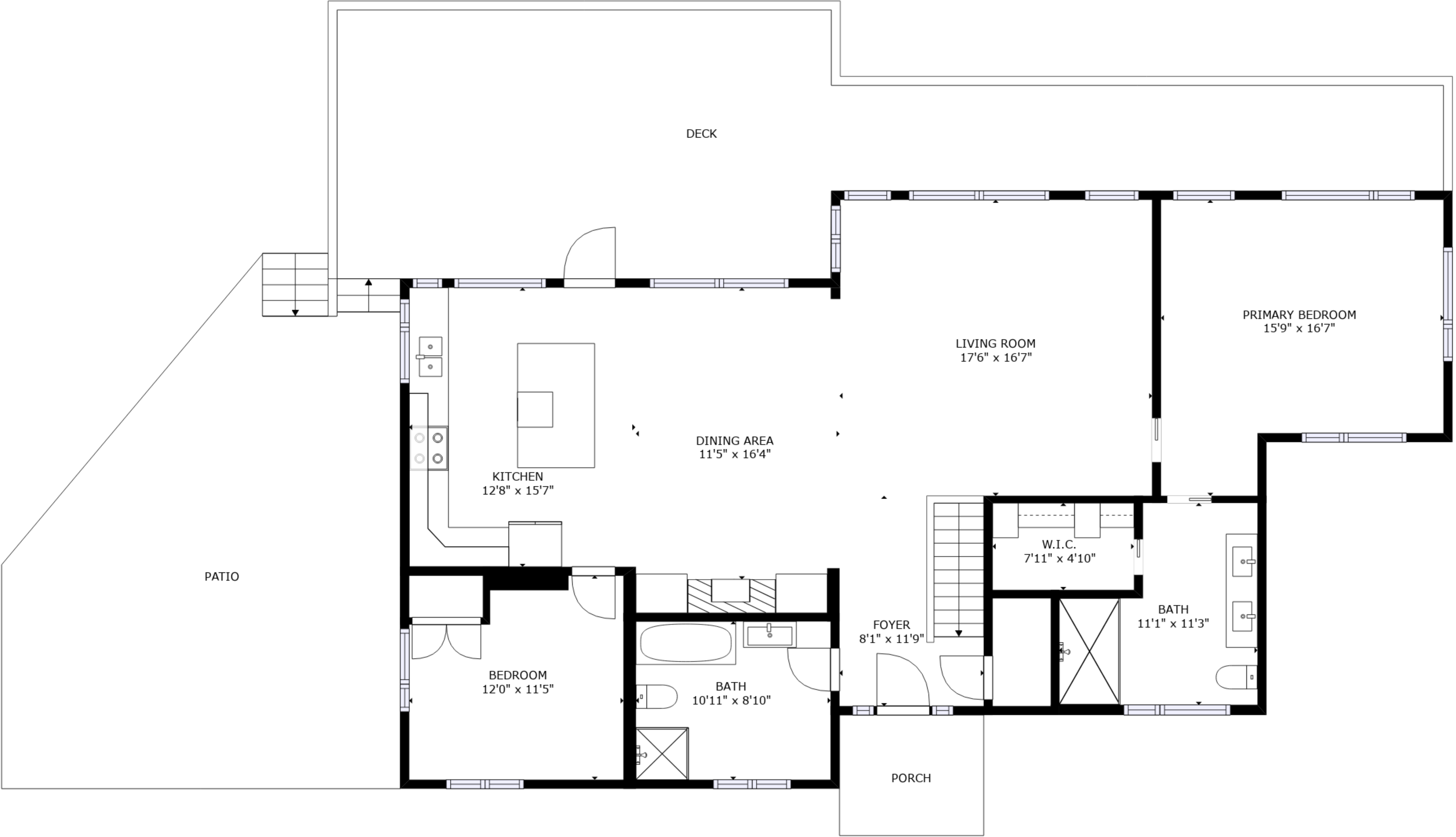
FLOOR 2
