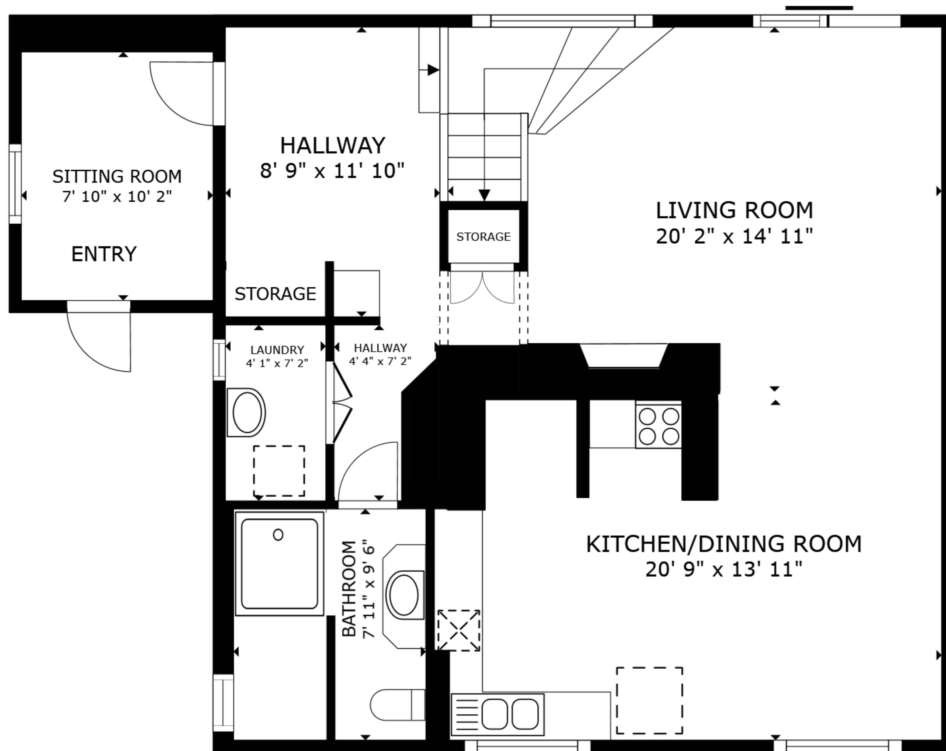
FLOOR 1
