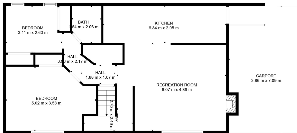
FLOOR 1
