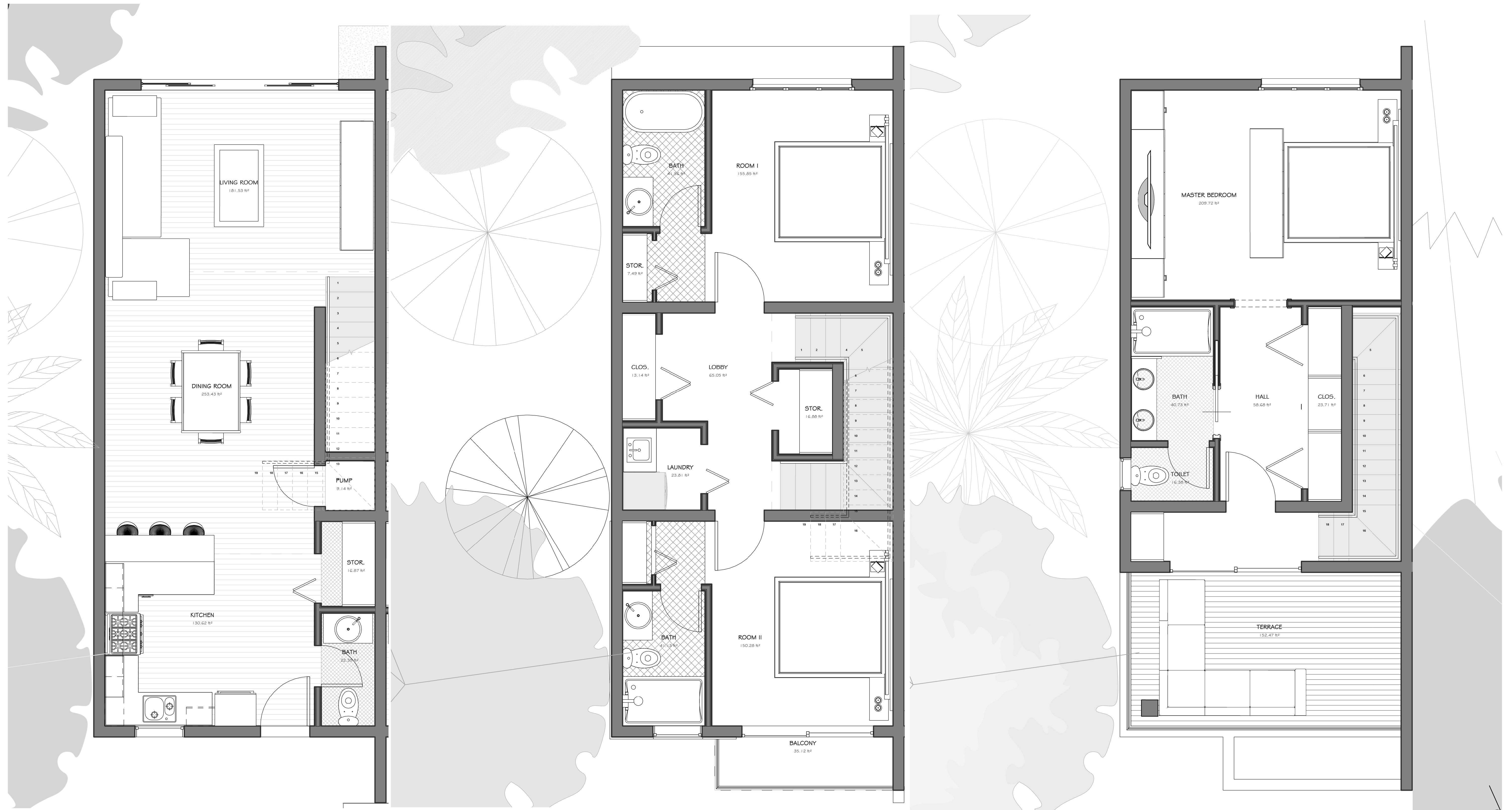
1 FIRST FLOOR PLAN A106. 3/8" = 1'-0"
