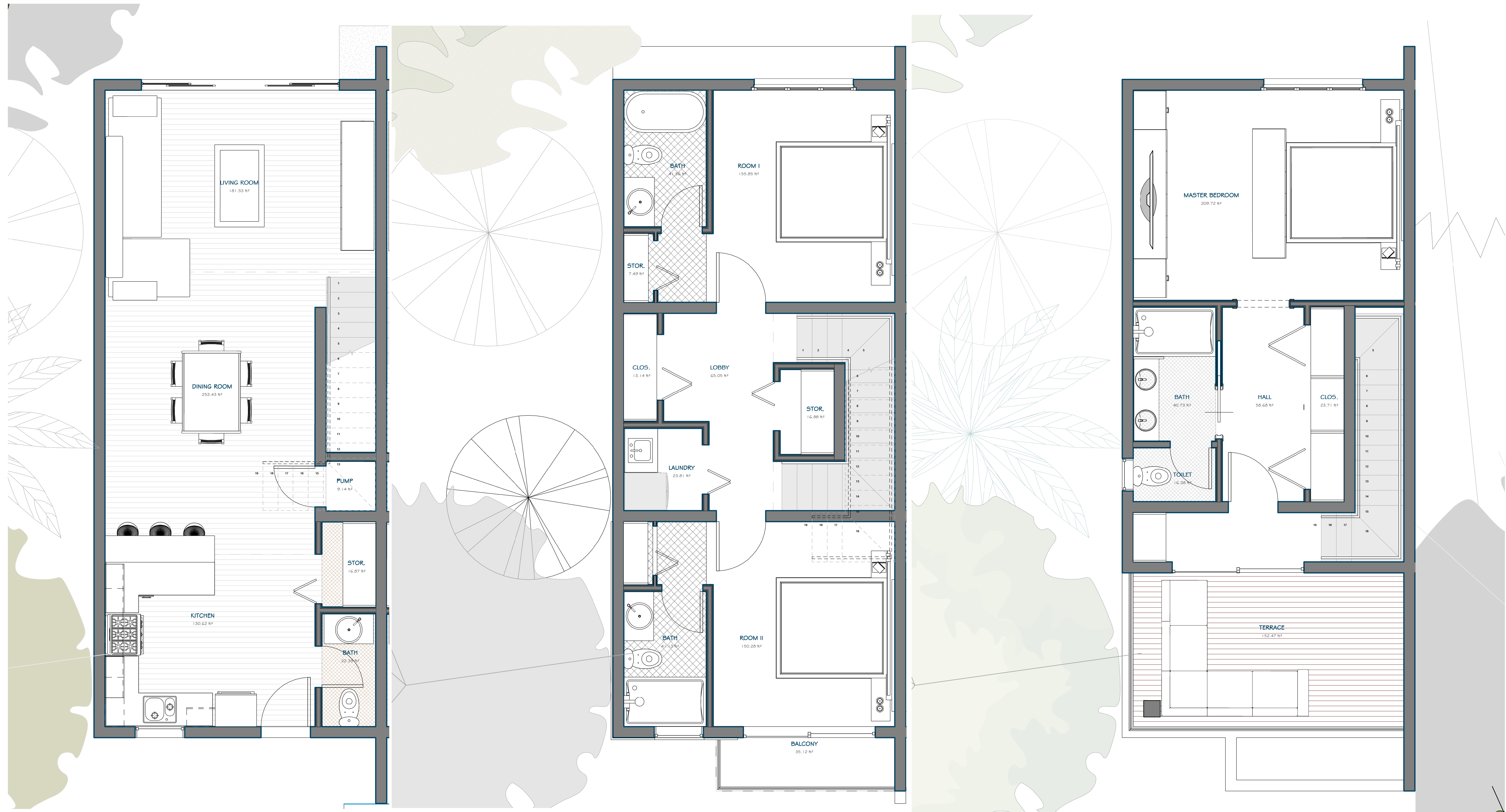
1 FIRST FLOOR PLAN A106. 3/8" = 1'-0"
