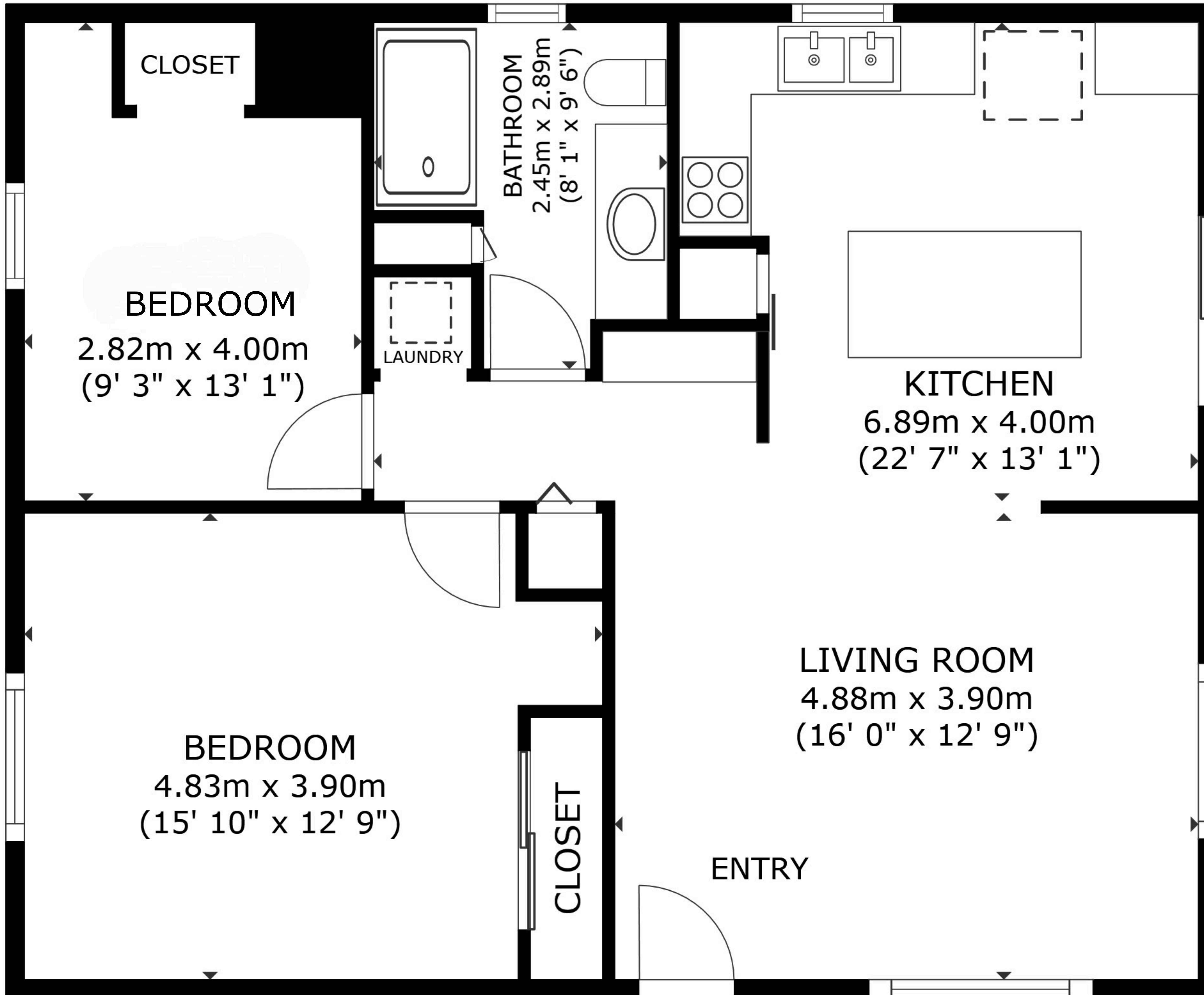
FLOOR PLAN
