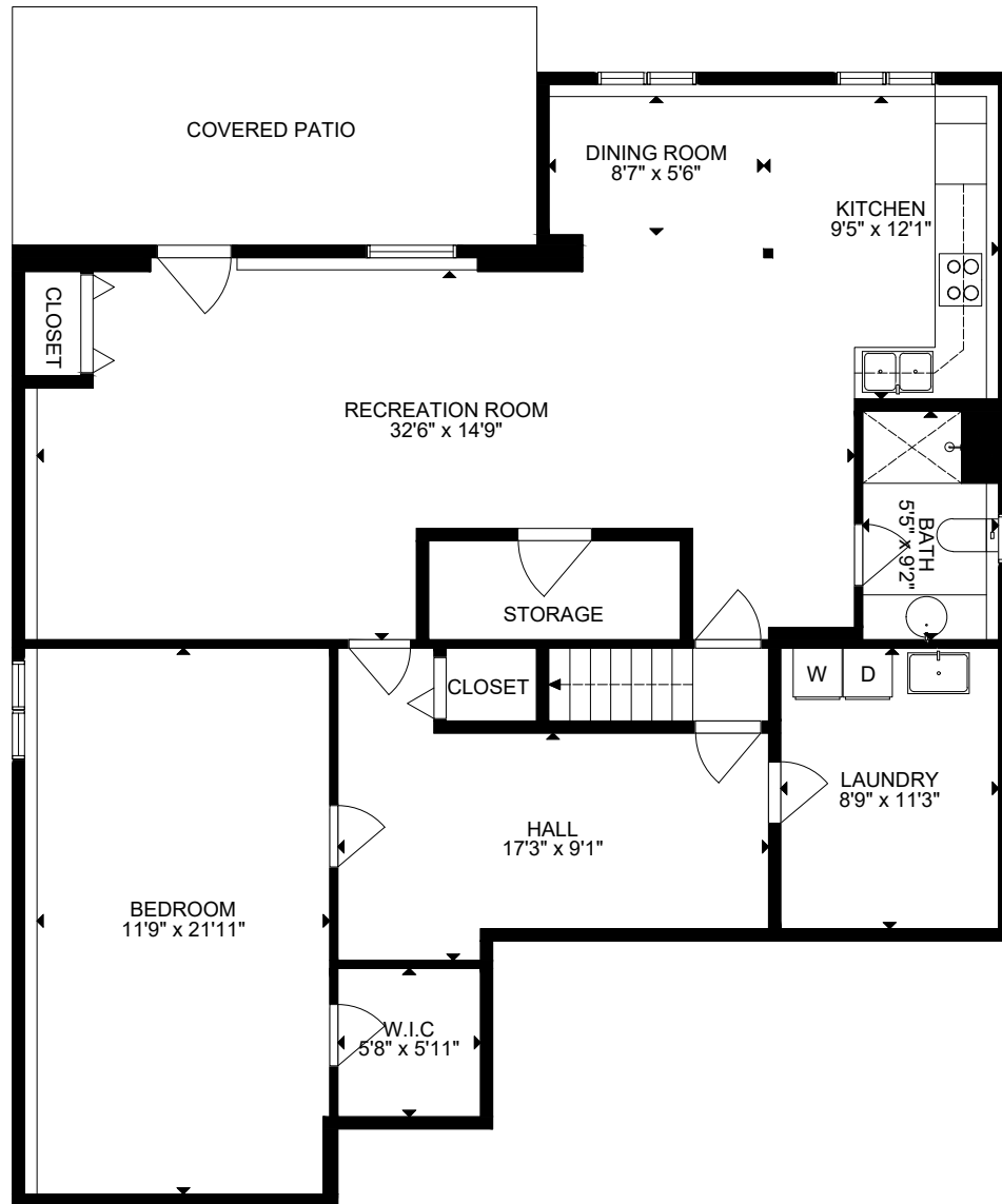
FLOOR 1
