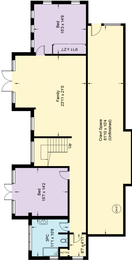
Lower Floor - 2238 sq ft
