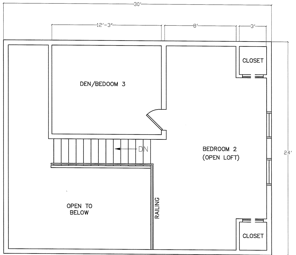
UPPER LEVEL FLOOR PLAN
