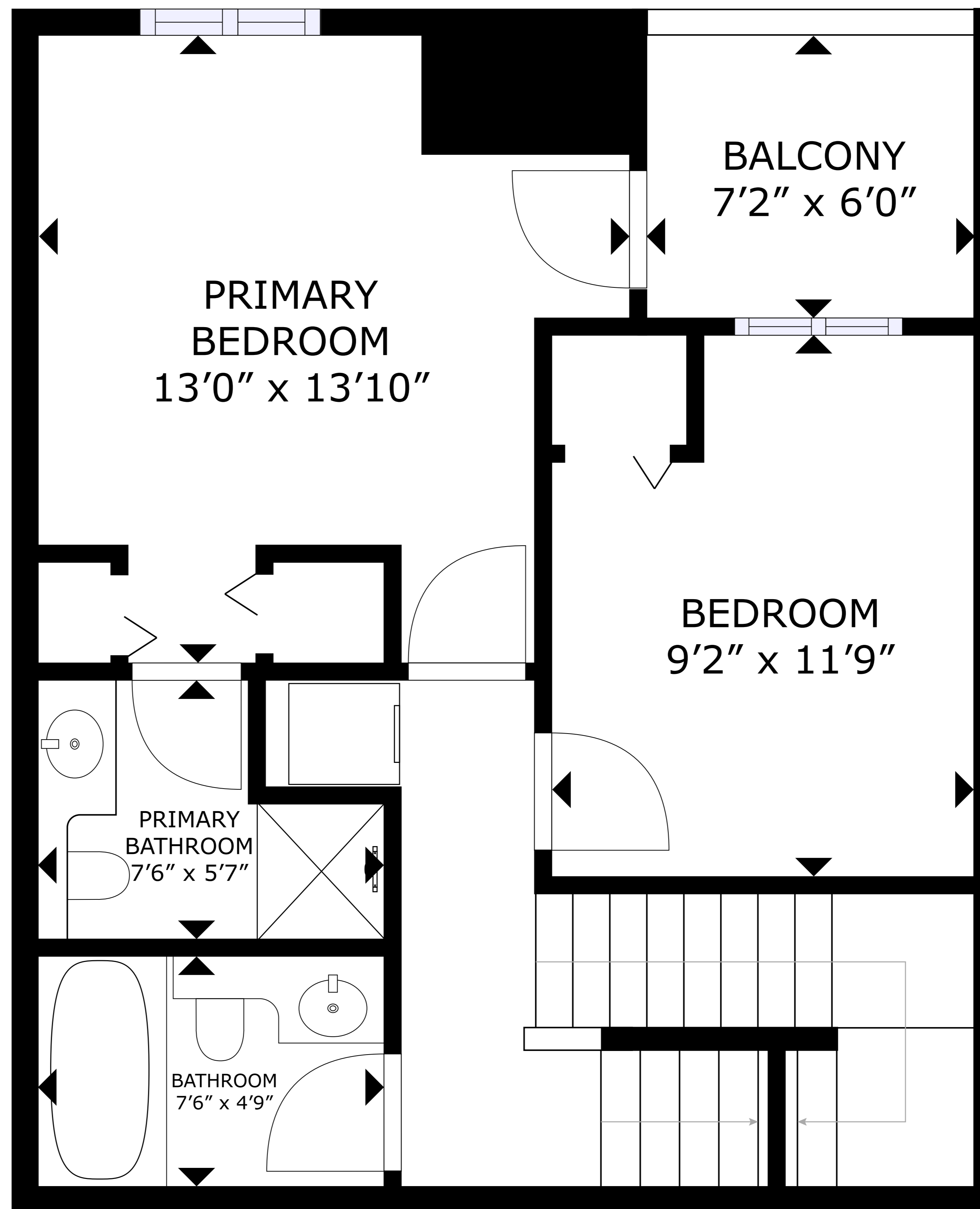
2ND FLOOR
