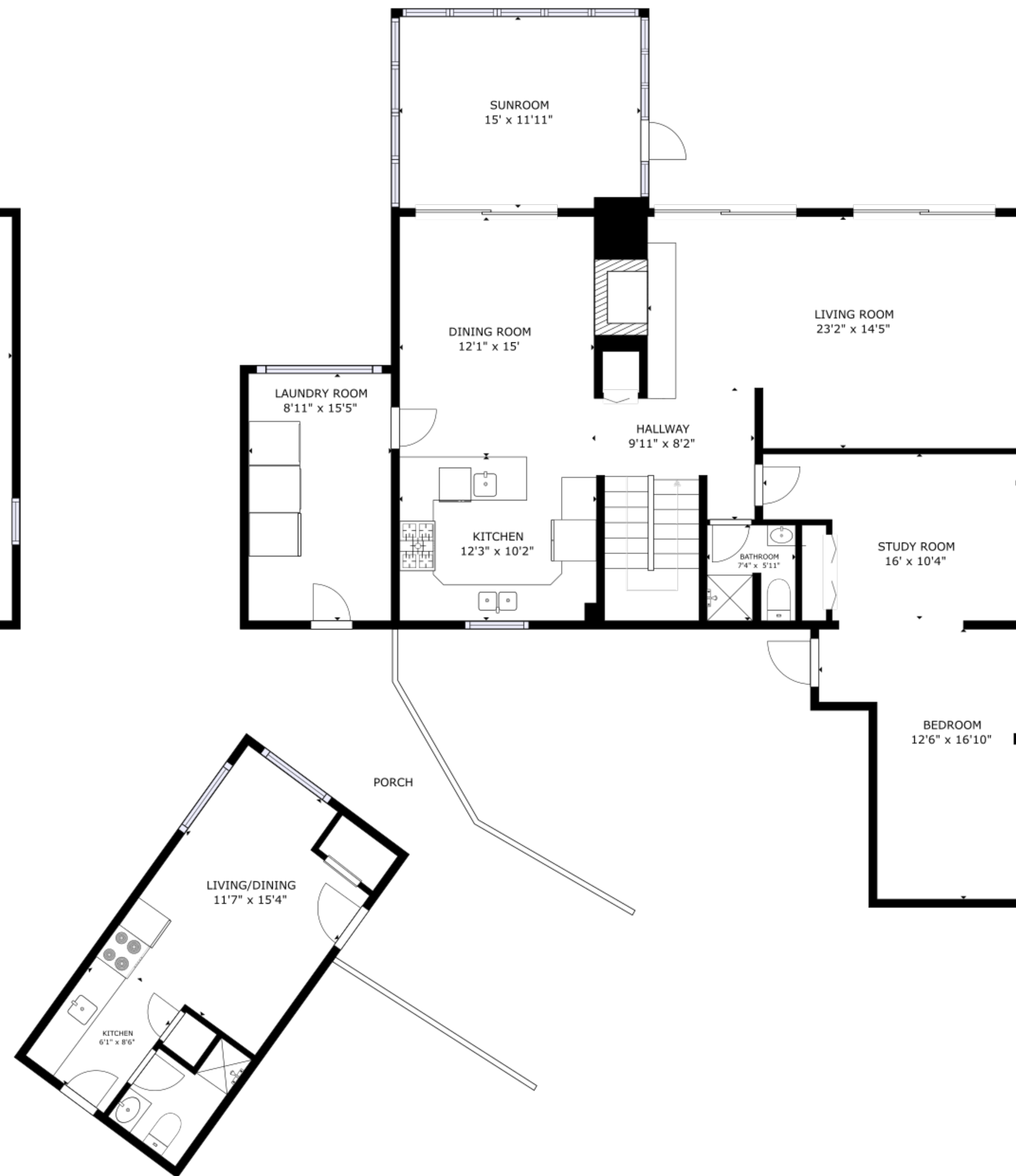
FLOOR 2
