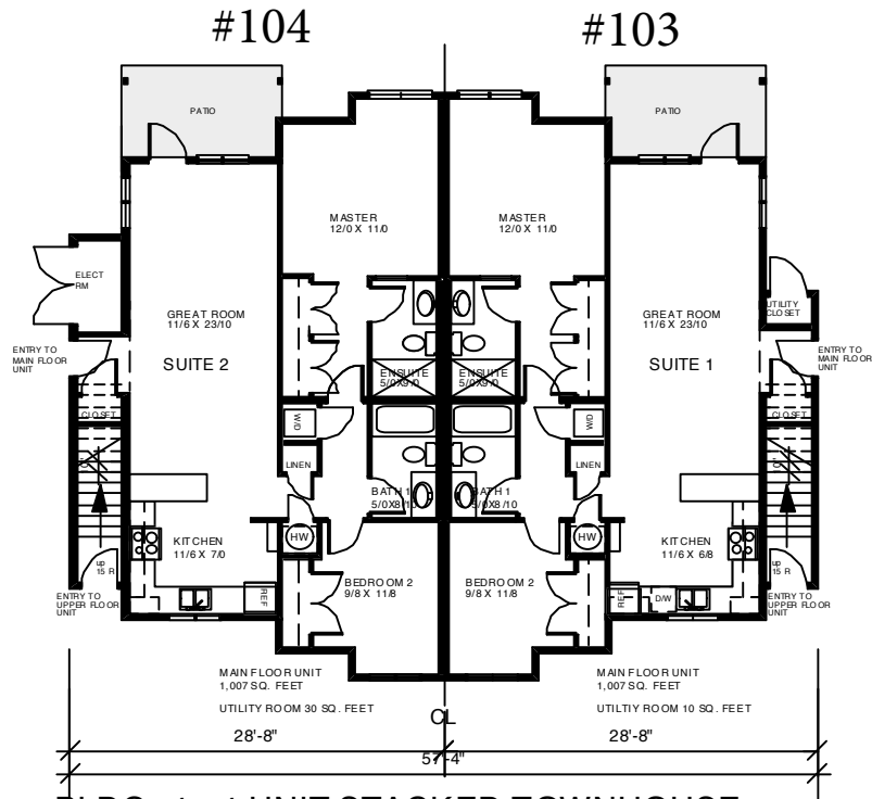
BLDG. 4 - 4 UNIT STACKED TOWNHOUSE MAIN FLOOR PLAN SCALE 1/16"=1'-0"
