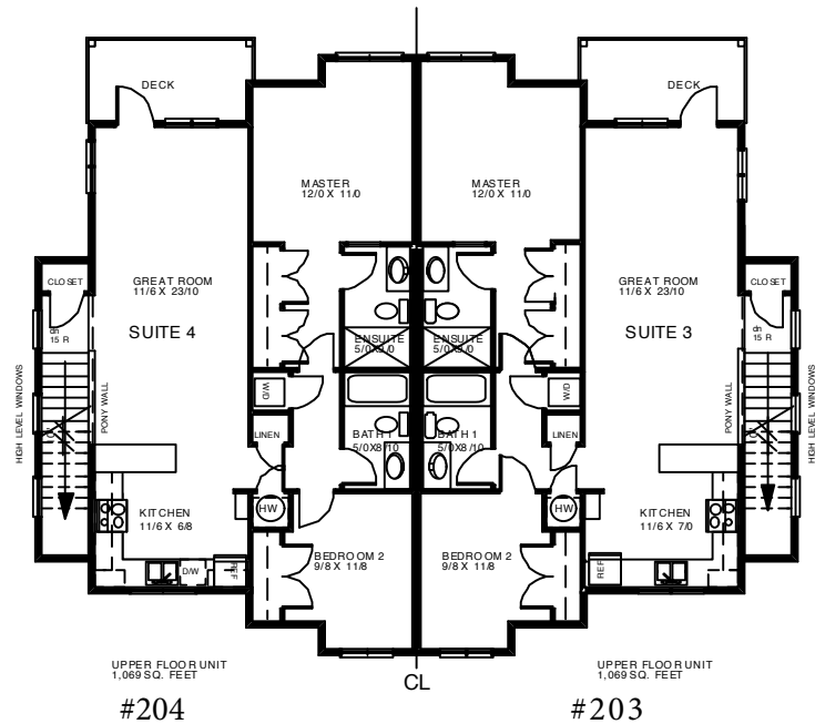
BLDG. 4 - 4 UNIT STACKED TOWNHOUSE UPPER FLOOR PLAN SCALE 1/16"=1'-0"
