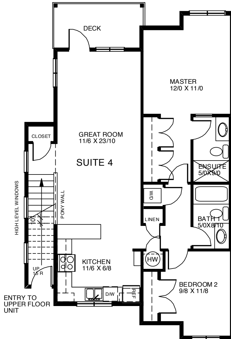
BUILDING 4 - 4 UNIT TOWNHOUSE TYPICAL UPPER FLOOR UNIT PLAN (REVERSE FOR OTHER SIDE)
