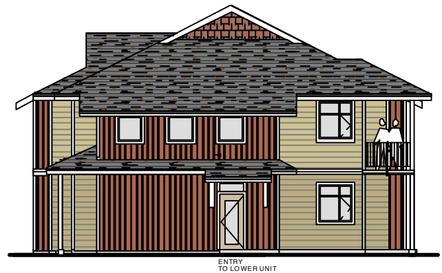
BLDG 4 STACKED TOWNHOUSE - RIGHT SIDE ELEVATION SCALE 1/16"=1'-0"
