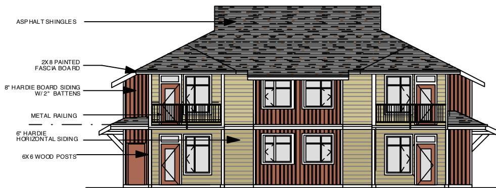
BLDG 4 STACKED TOWNHOUSE - REAR ELEVATION
