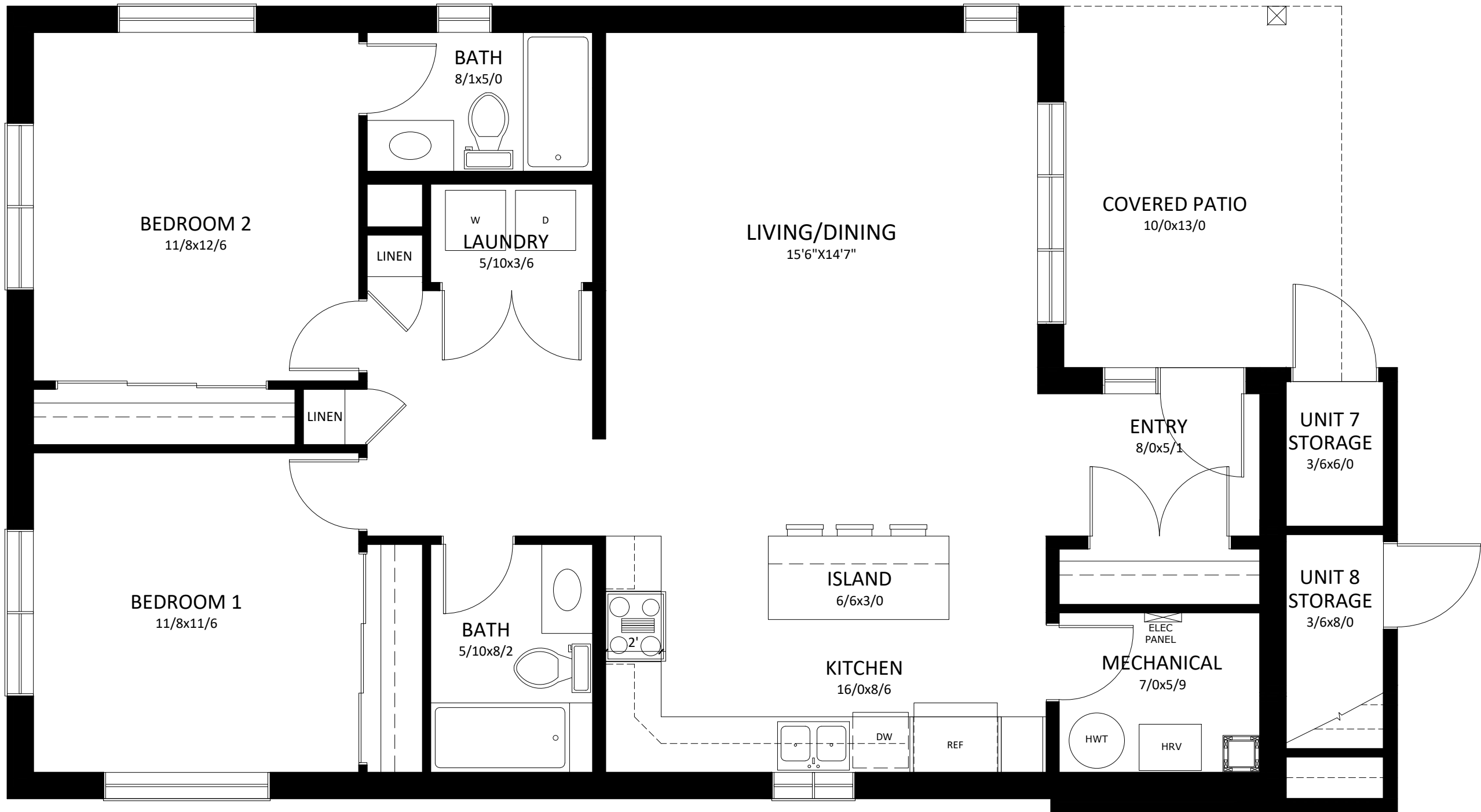
MAIN FLOOR PLAN - UNIT 7 SCALE: AS SHOWN
