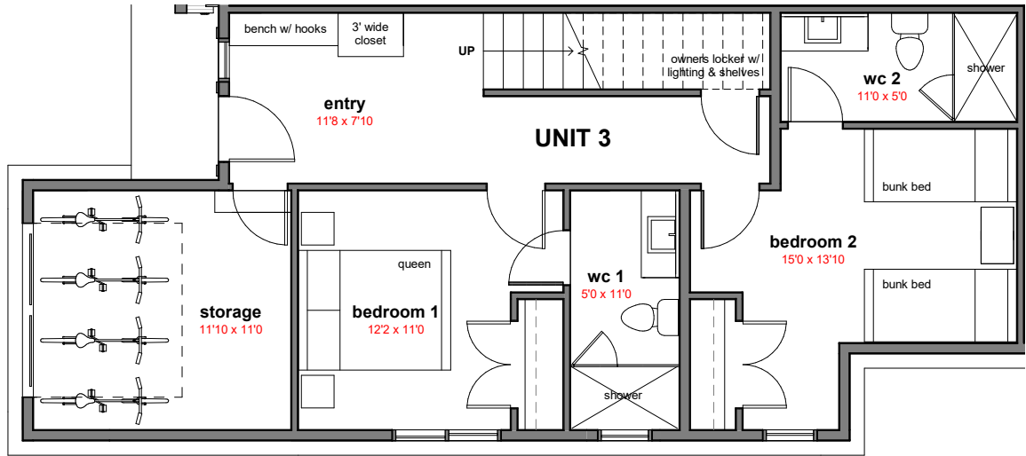
first floor plan 759.61ft 2
