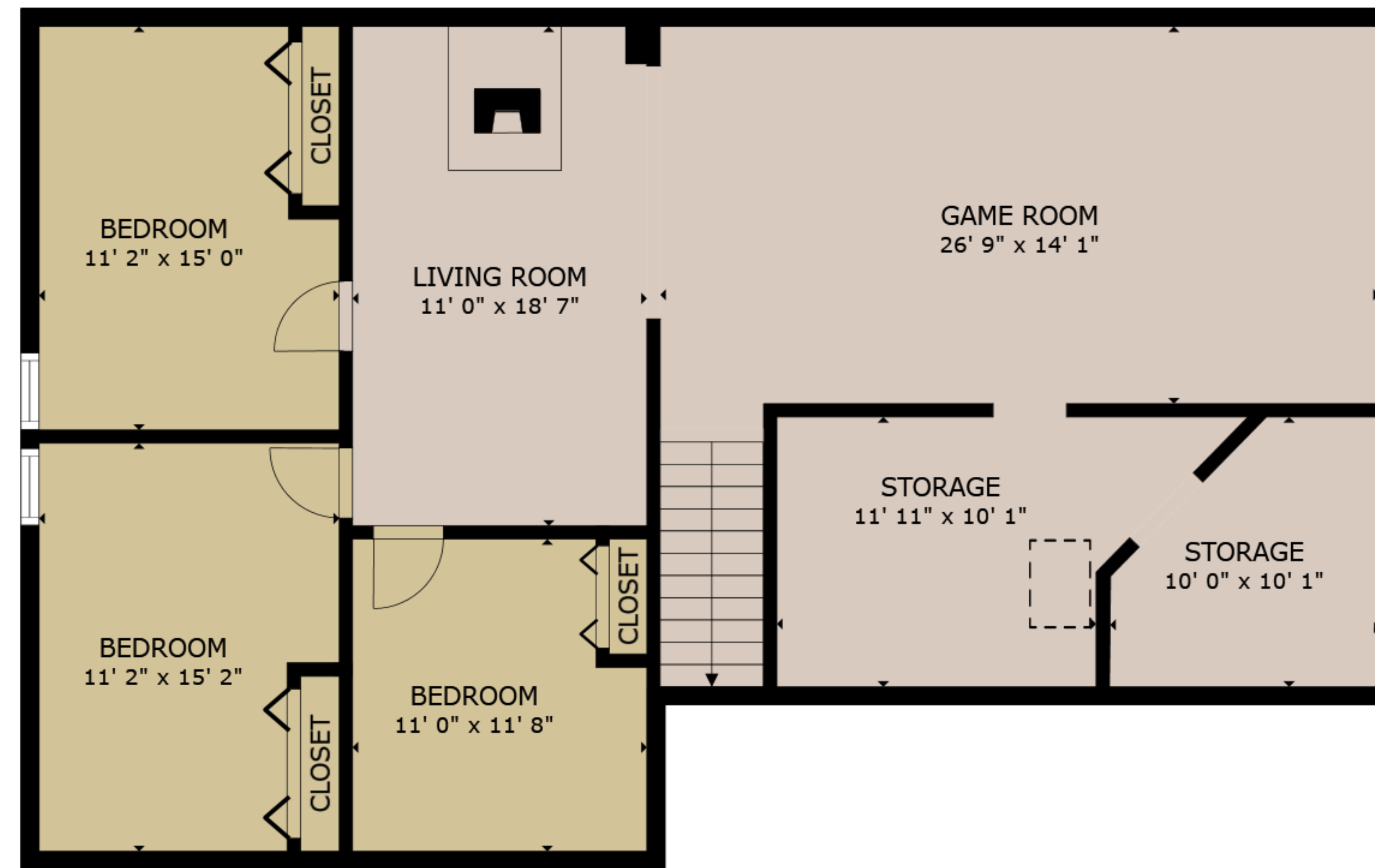
FLOOR 1
