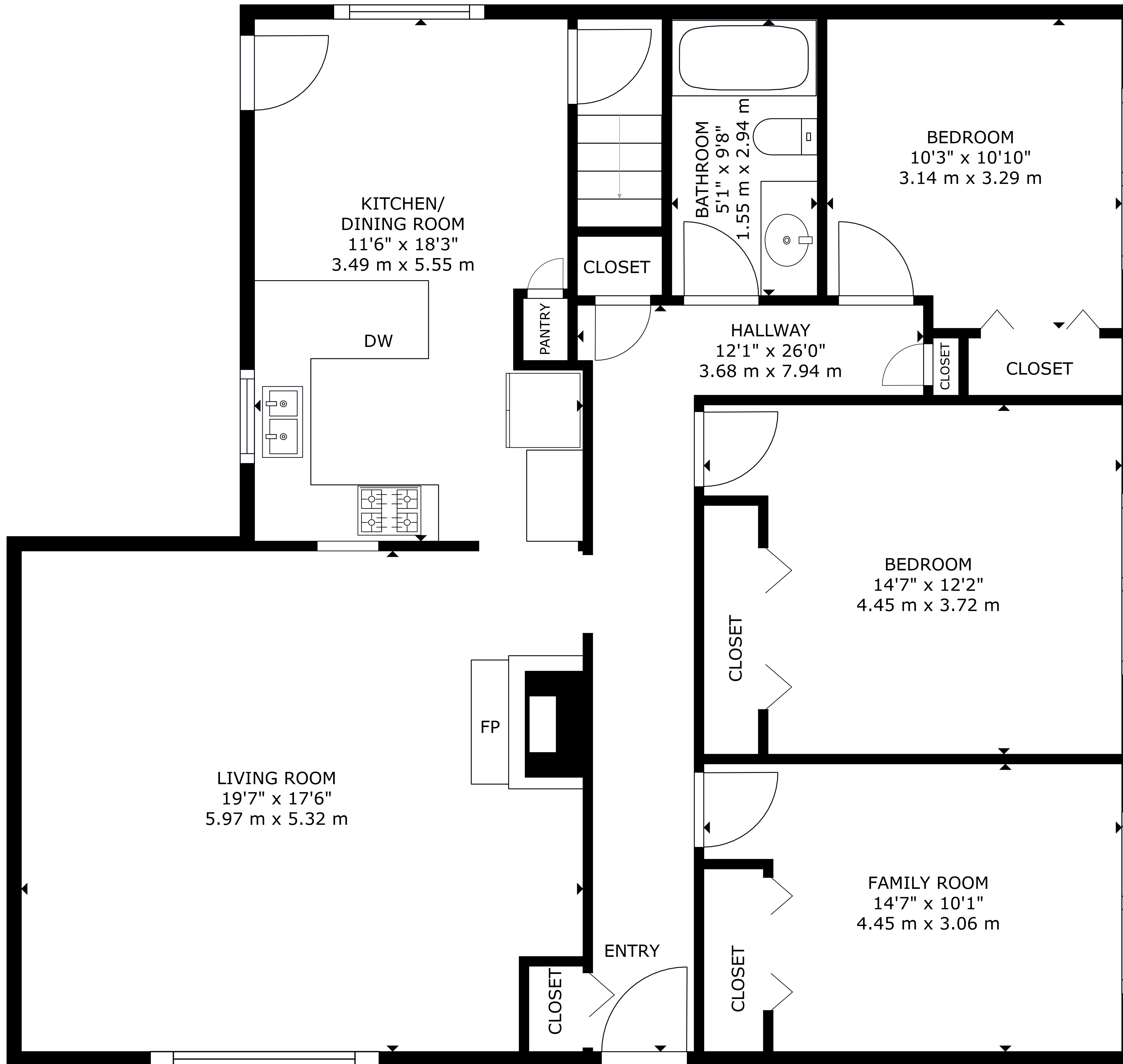
FLOOR PLAN
