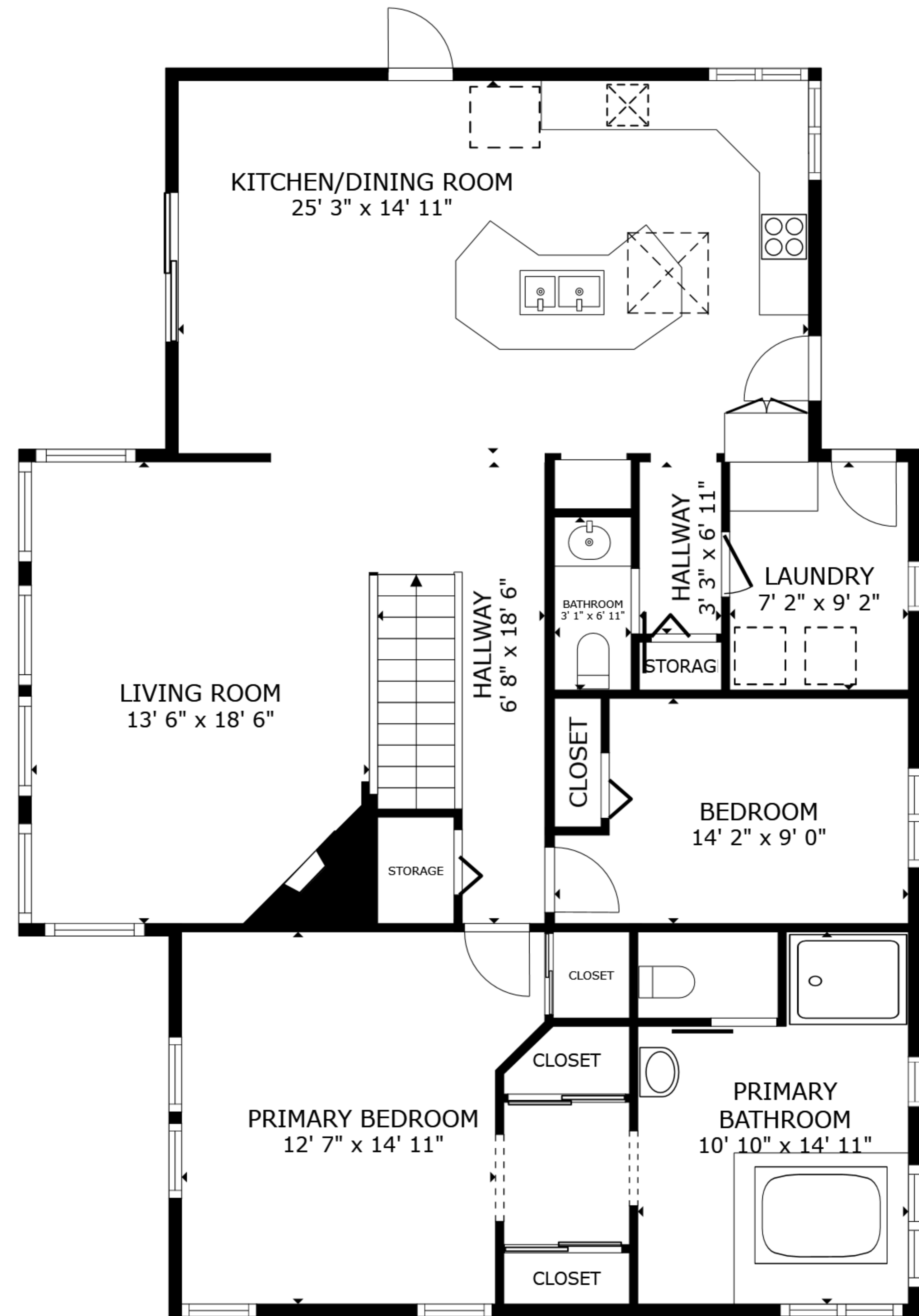
FLOOR 2
