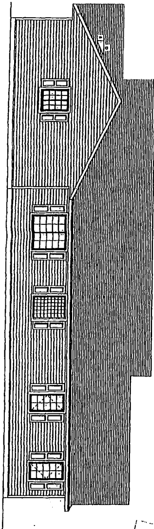
Rear Elevation Scale 1/8" = 1'-0"
