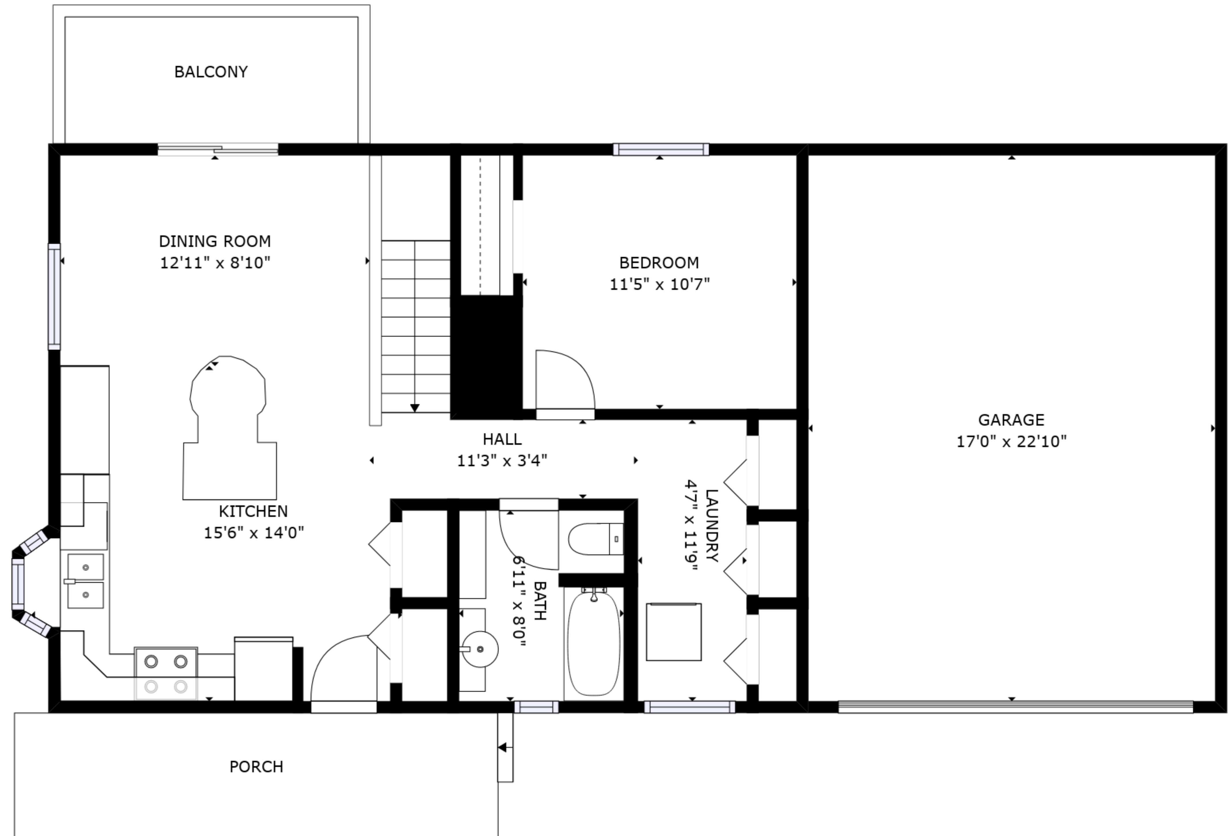
FLOOR 2
