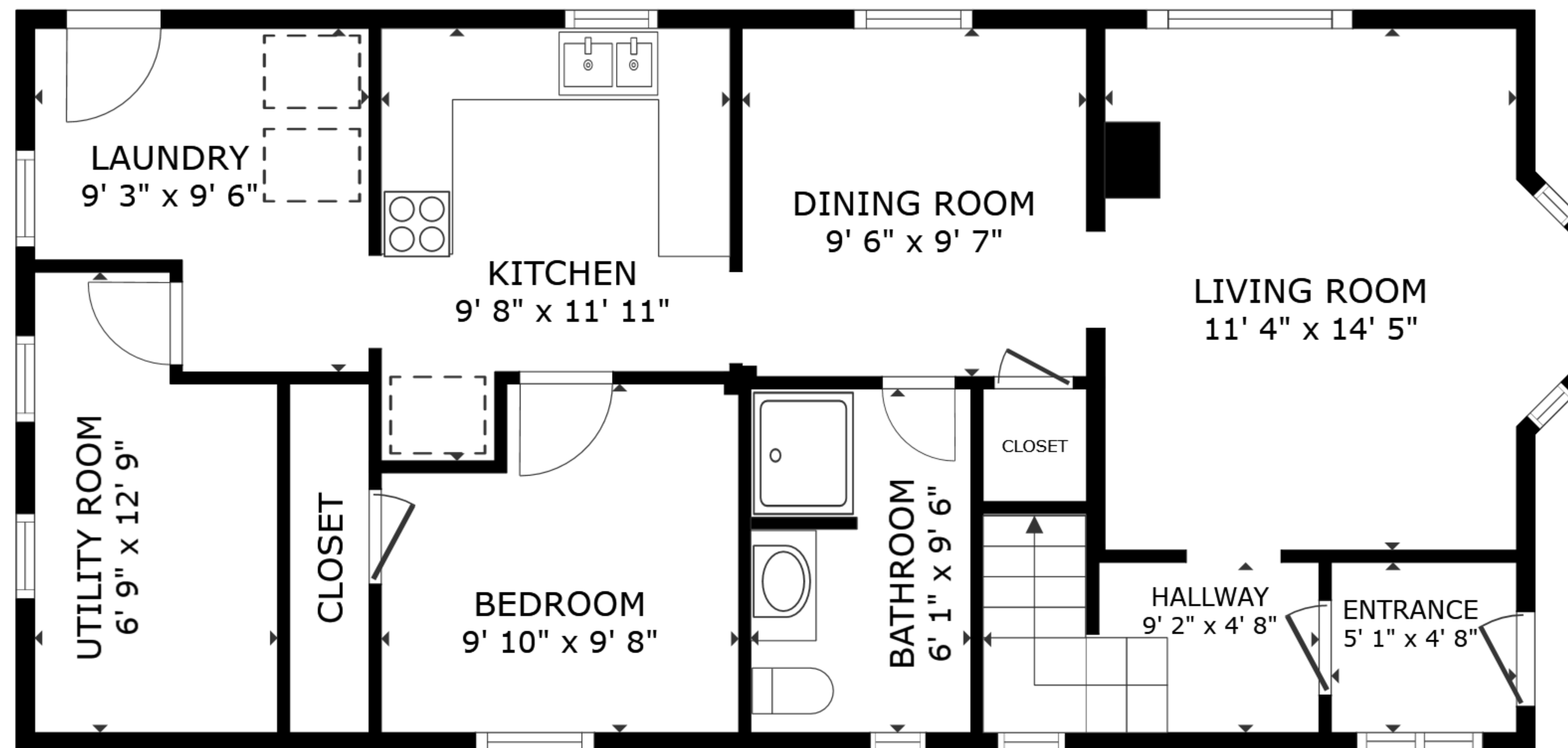
FLOOR 1
