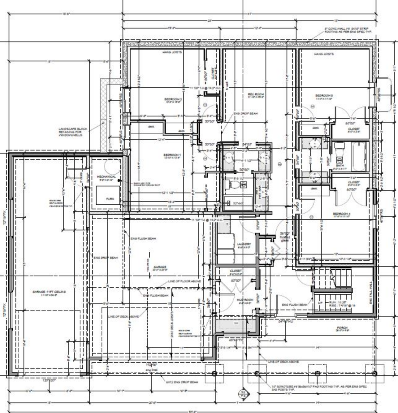
LOWER FLOOR PLAN SCALE: 1/4" = 1' - 0"
